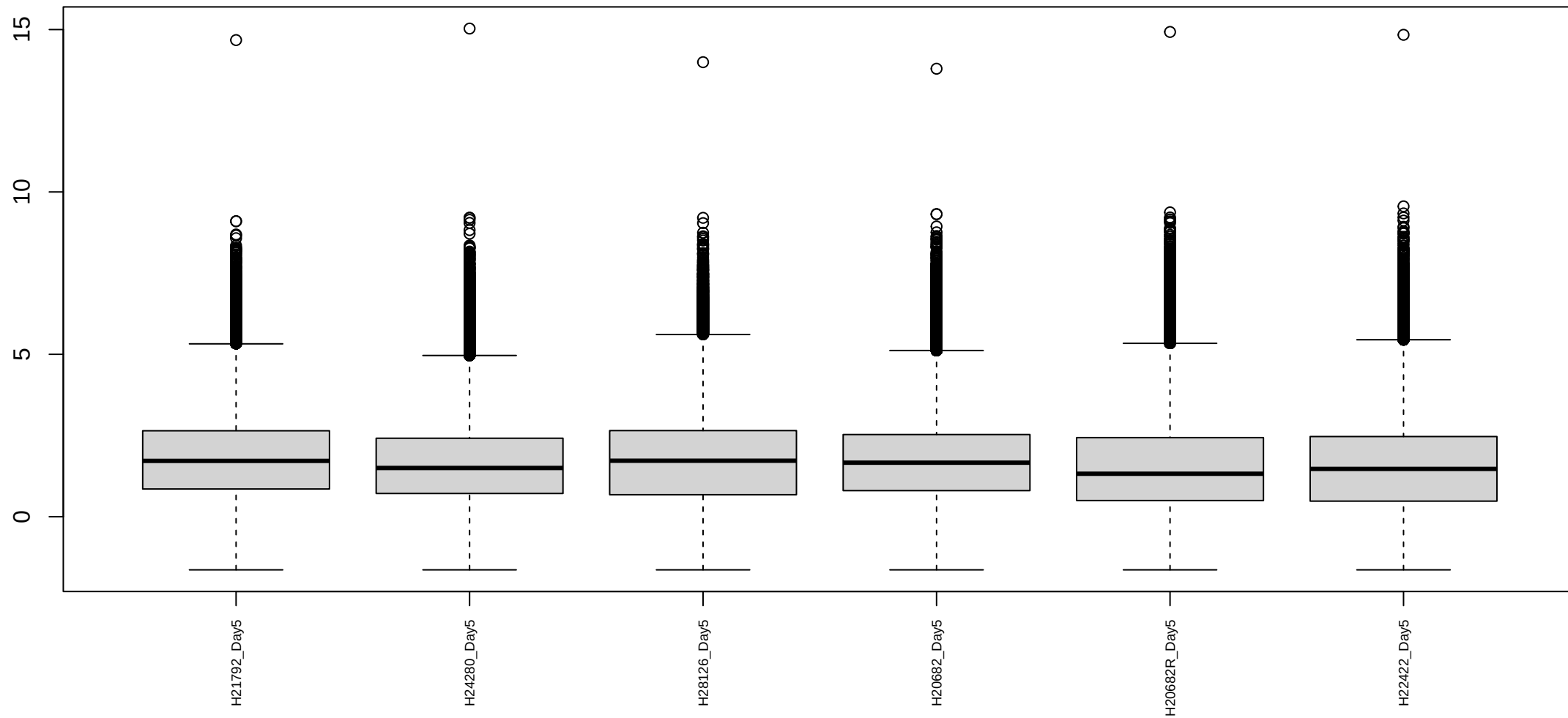
Boxplots of log cpm per sample Human Day 5 Reproducible3
