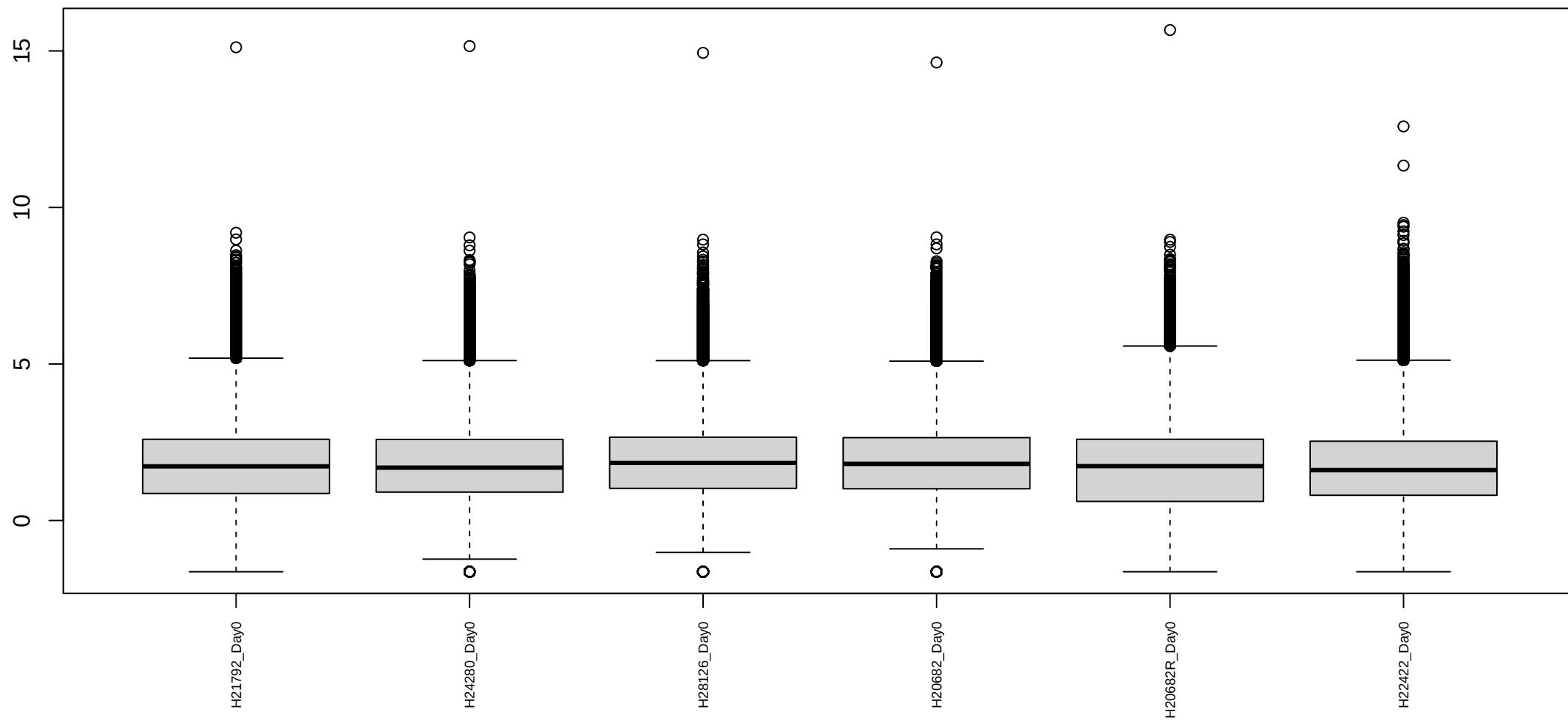
Boxplots of log cpm per sample Human Day 0 Reproducible3
