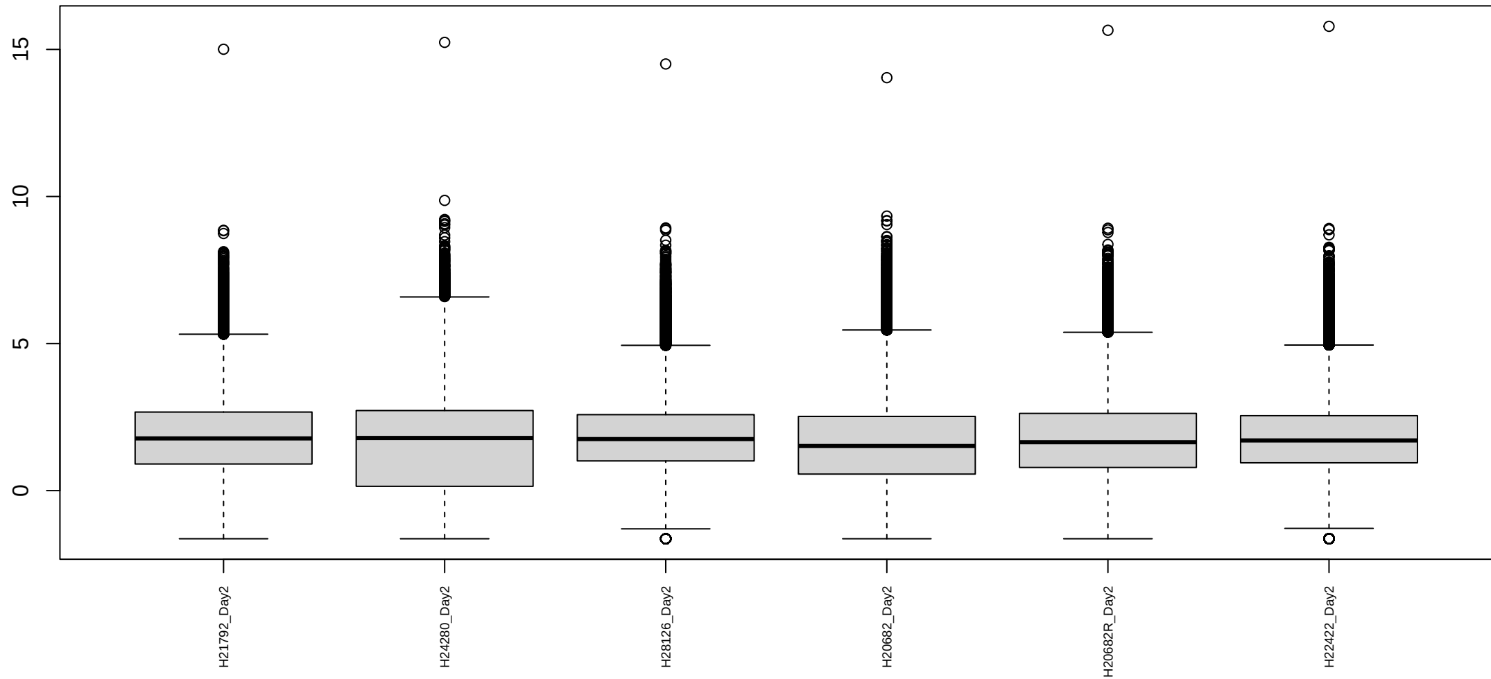
Boxplots of log cpm per sample Human Day 2 Reproducible3
