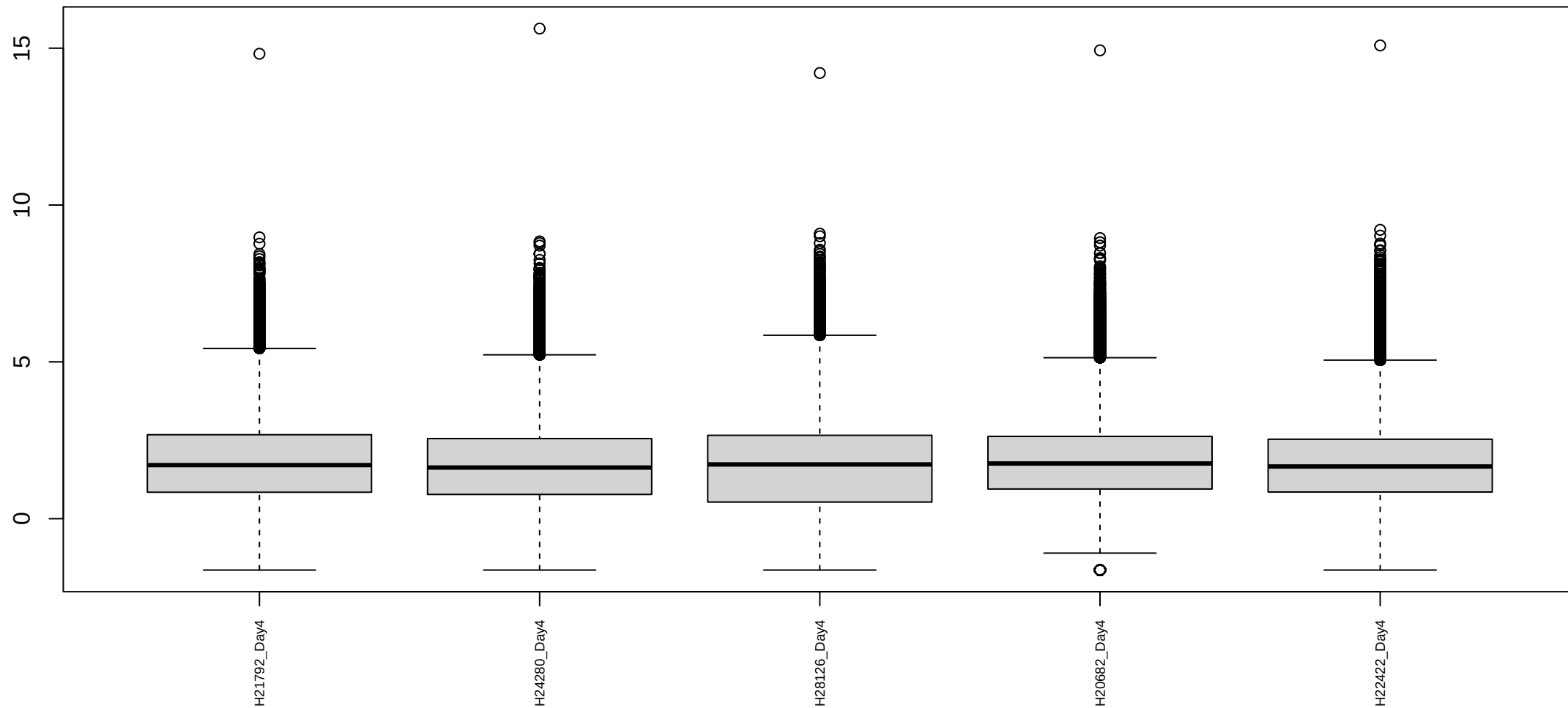
Boxplots of log cpm per sample Human Day 4 Reproducible3
