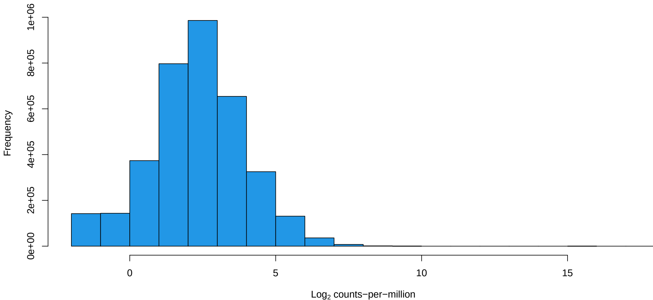
Histogram of all counts – Human Reproducible4
