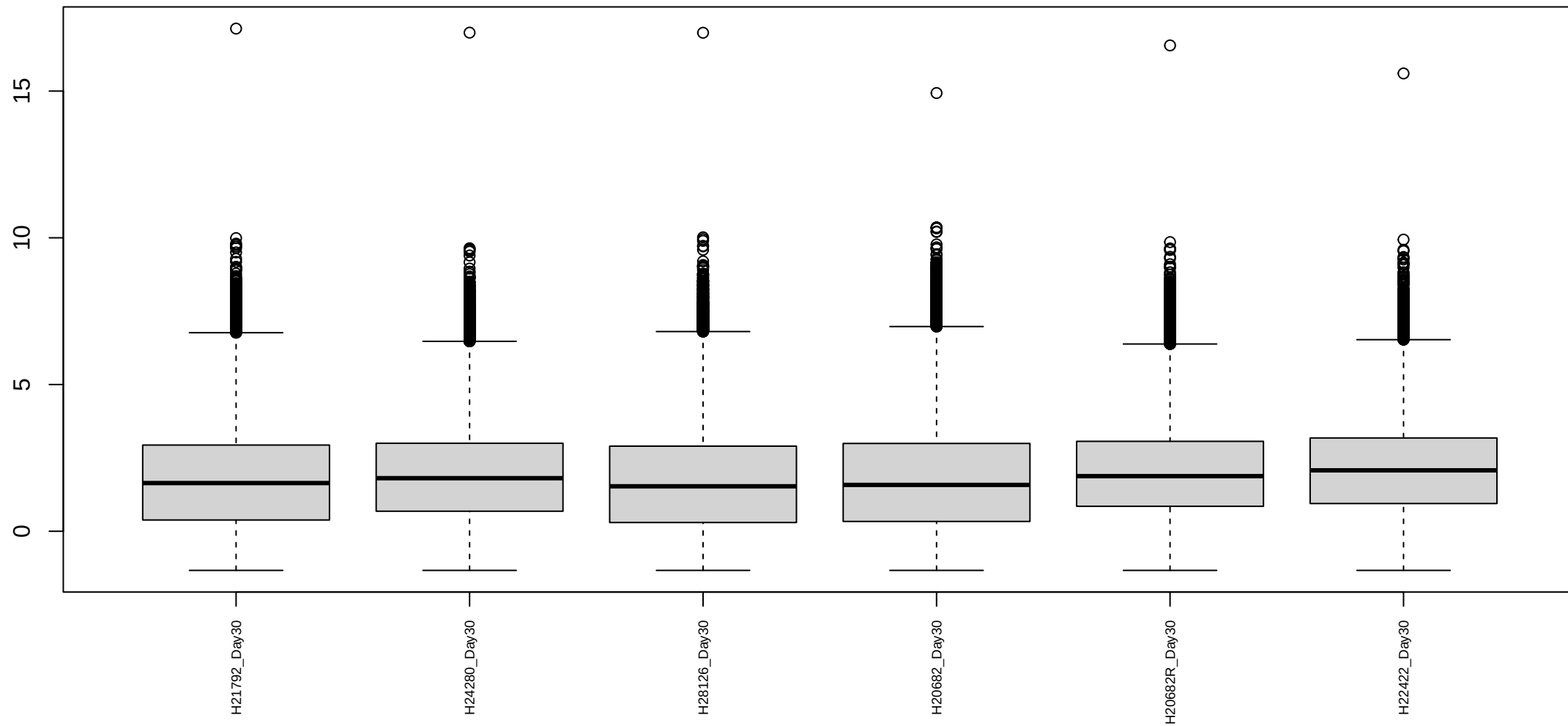
Boxplots of log cpm per sample Human Day 30 Reproducible4
