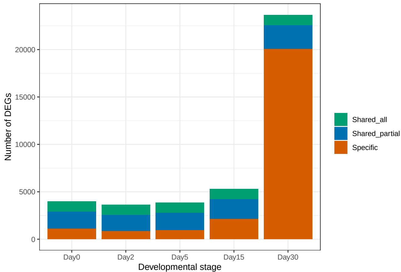
Fate of HvC DEGs across development
