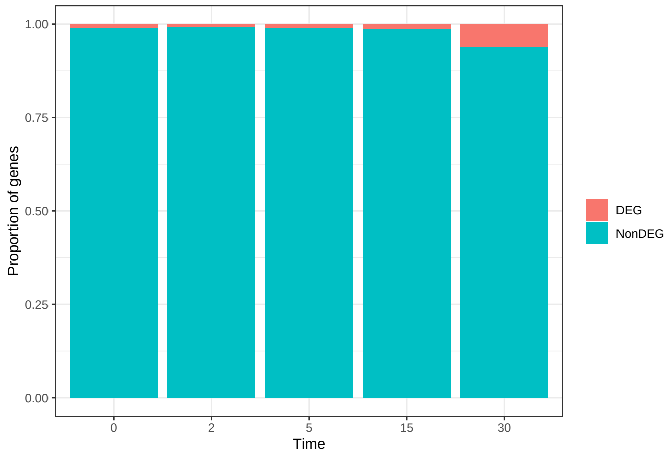
HvC comparisons: DEG vs NonDEG composition
