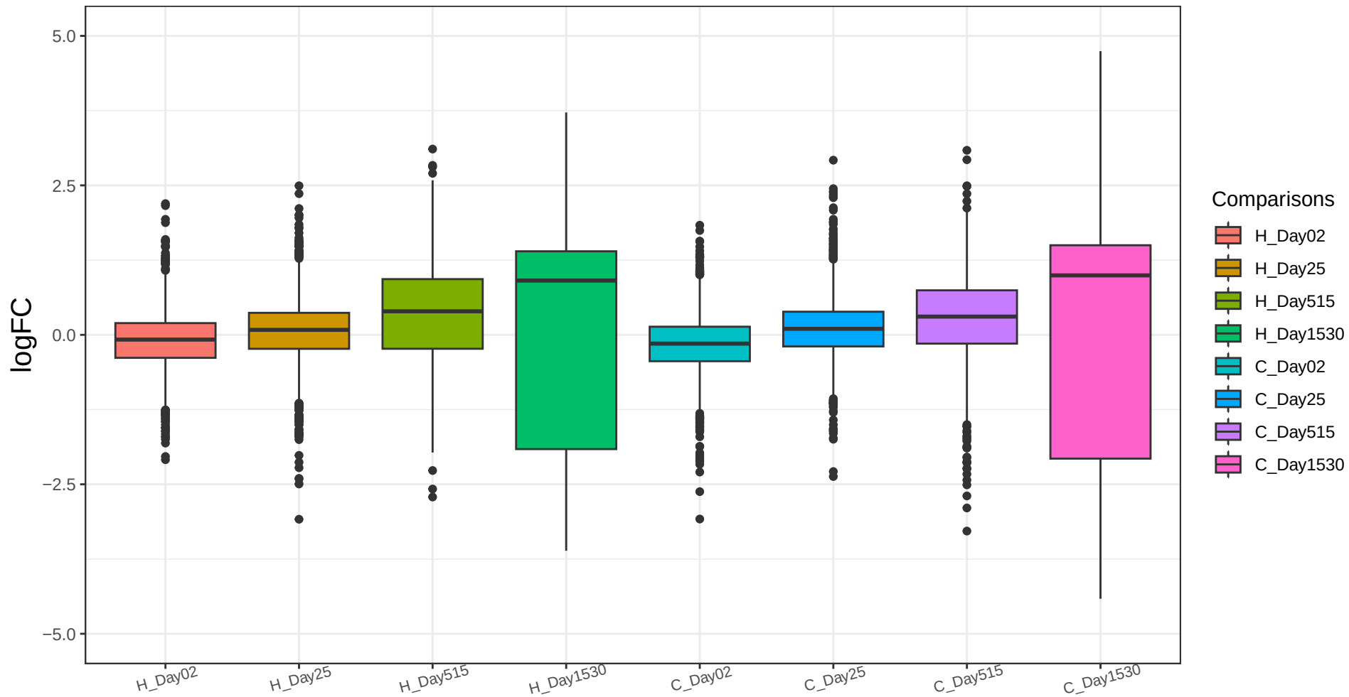
Traj1530_genes Trajectory DEG FC Comparisons Kruskal-Wallis p = 1.18e-148
