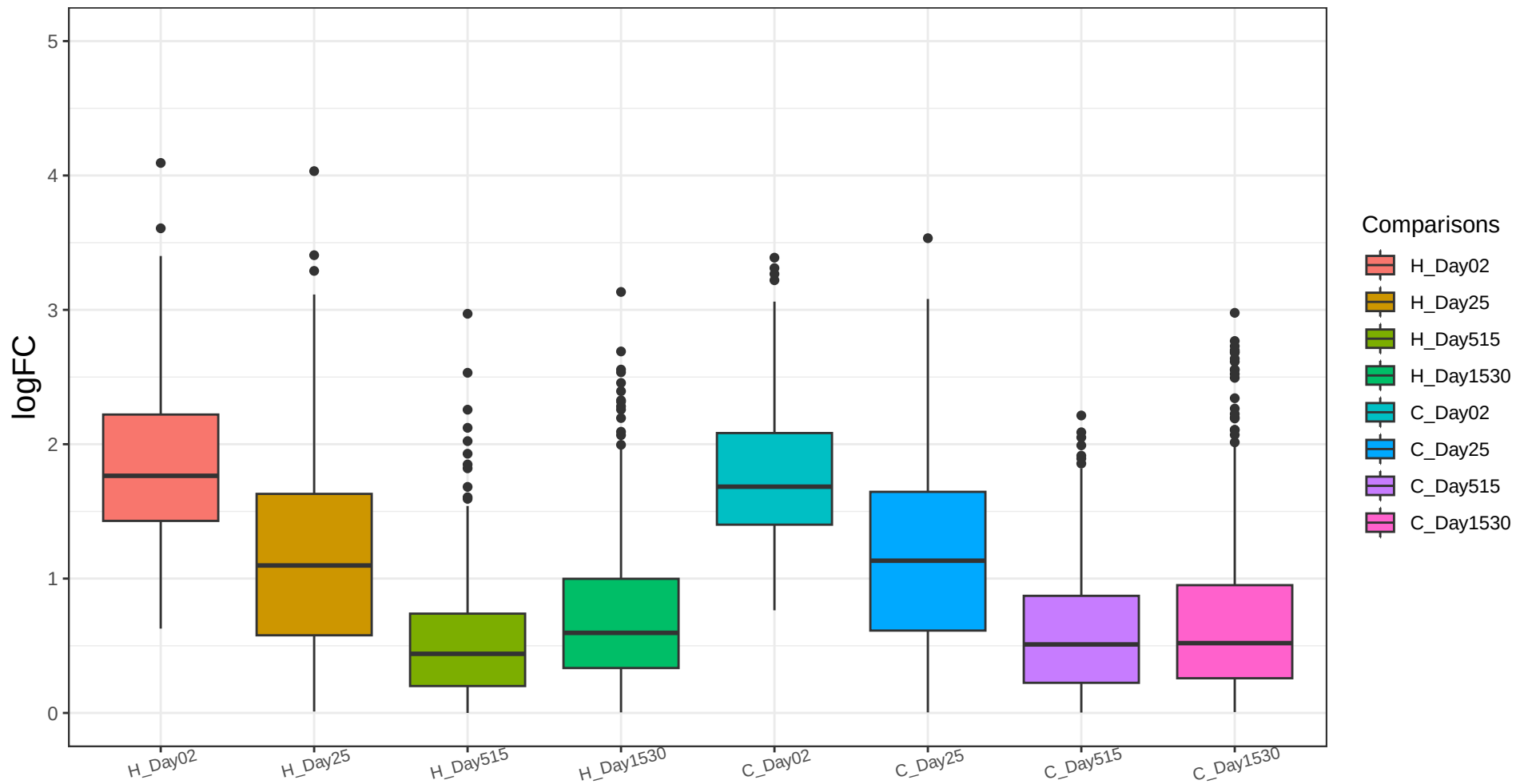
Traj02_genes Trajectory DEGs FC Comparisons Kruskal-Wallis p = 2.49\text{e-}157
