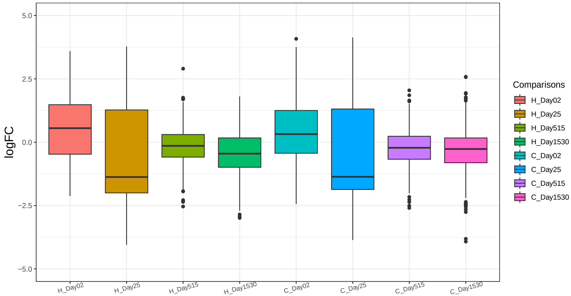
Traj25_genes Trajectory DEG FC Comparisons Kruskal-Wallis p = 5.75e-105
