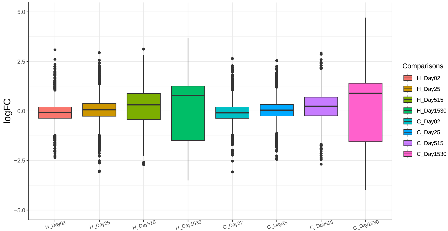
Traj1530_genes Trajectory DEG FC Comparisons Kruskal-Wallis p = 1.55e-161
