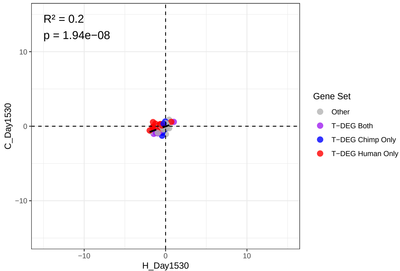
H_Day1530 vs C_Day1530 --All Expressed Genes
