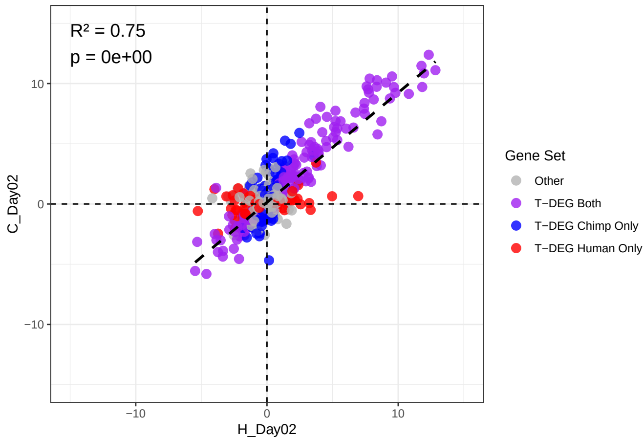
H_Day02 vs C_Day02 --All Expressed Genes
