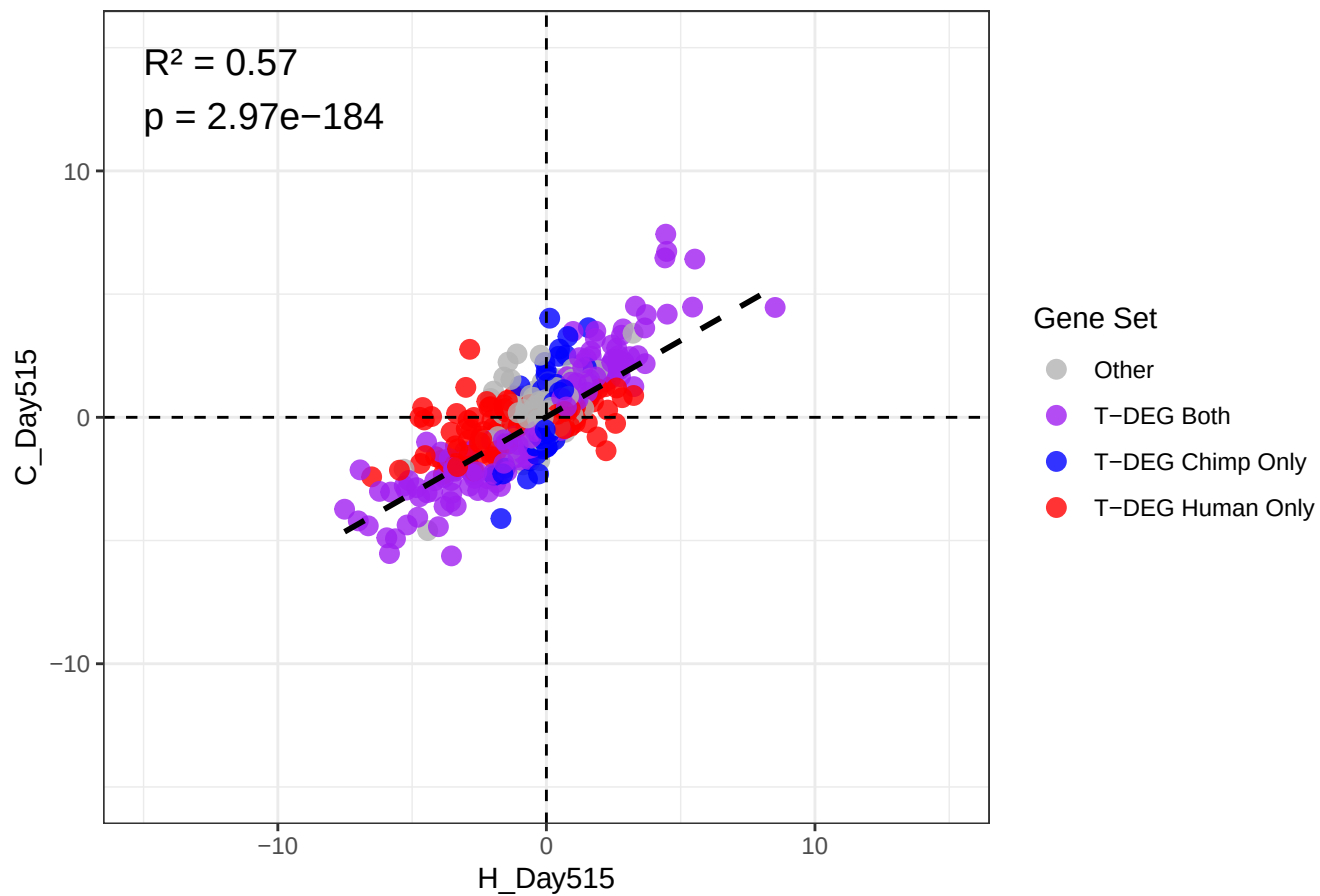
H_Day515 vs C_Day515 --All Trajectory DEGs
