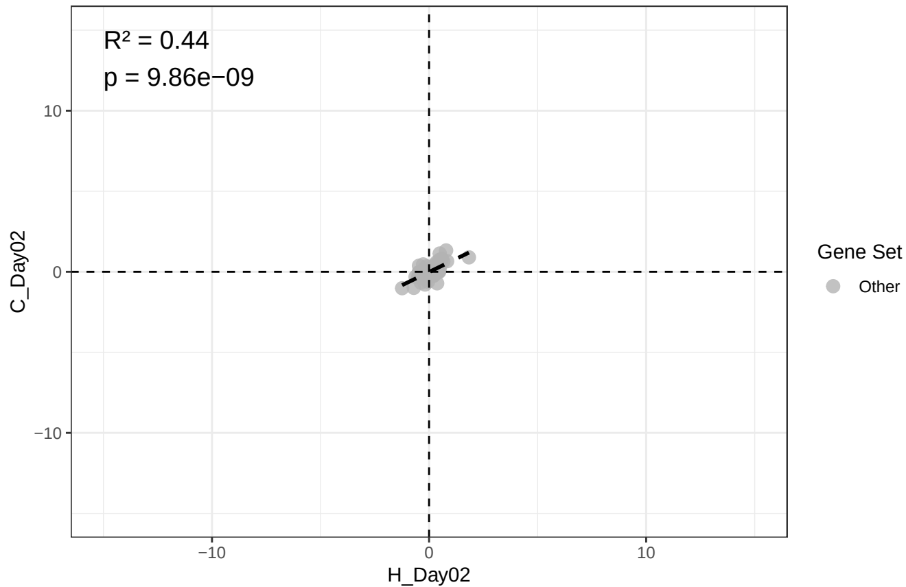
H_Day02 vs C_Day02 --Trajectory Non-DEGs (no Transitions)
