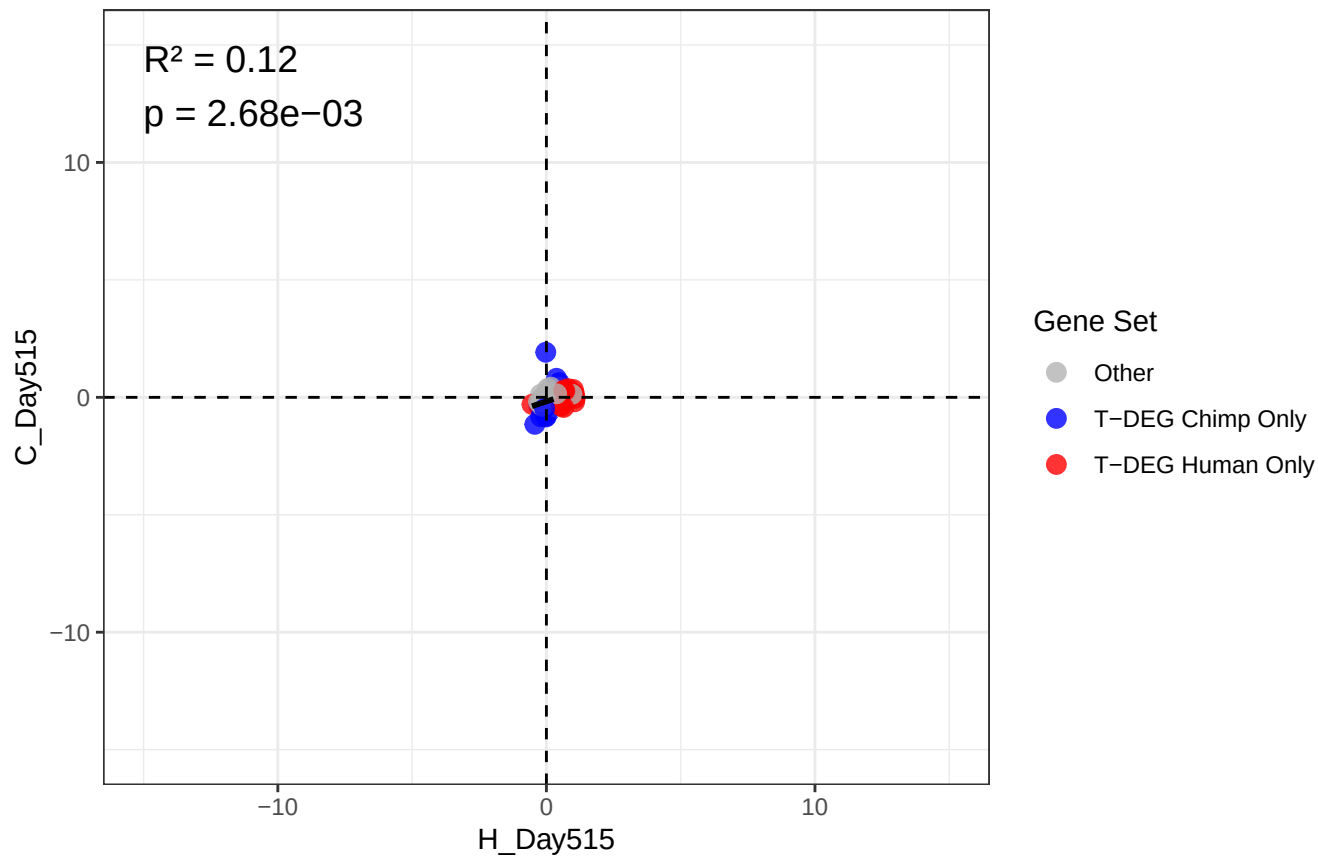
H_Day515 vs C_Day515 --TF Species-NonShared Trajectory DEGs (no Transitions)
