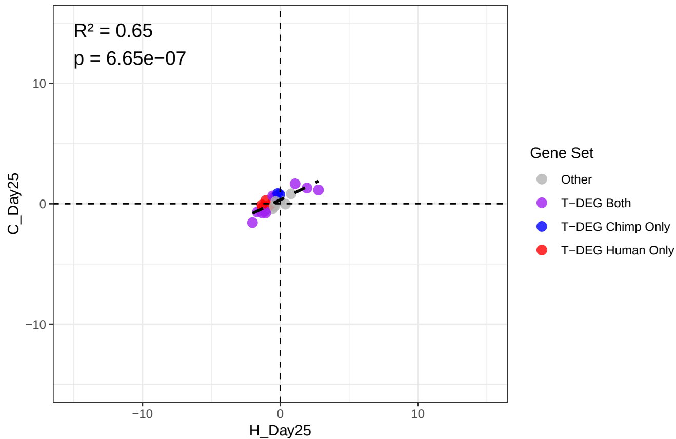
H_Day25 vs C_Day25 --Species-Shared Trajectory DEGs (at least on Transition)
