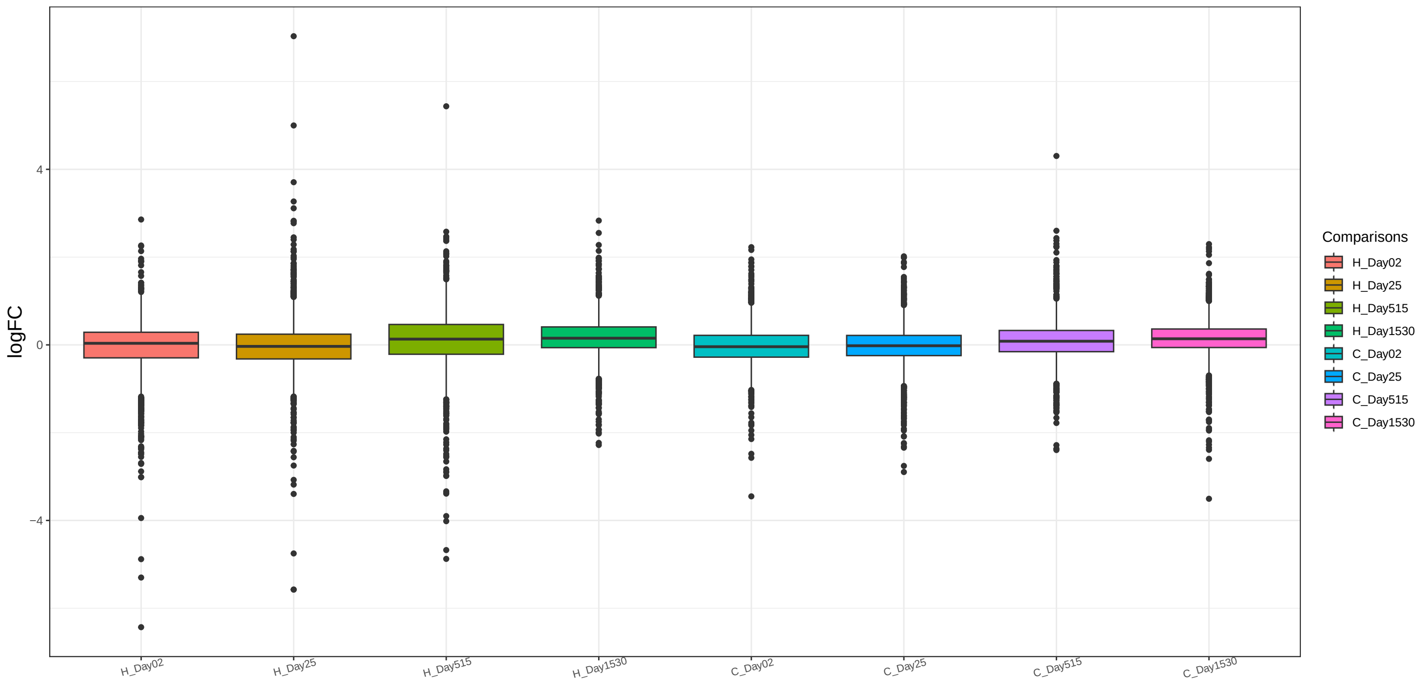
clust1 RNA FC Comparisons Kruskal-Wallis p = 5.63e-232
