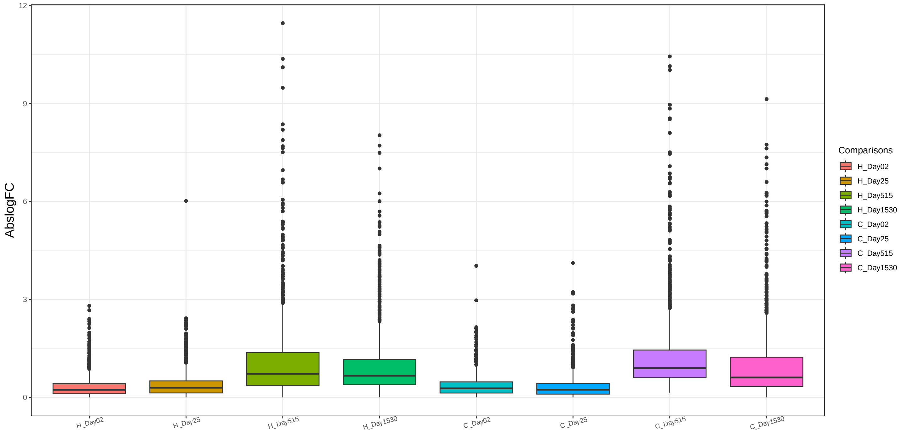
clust7 RNA AbsFC Comparisons Kruskal-Wallis p = 0
