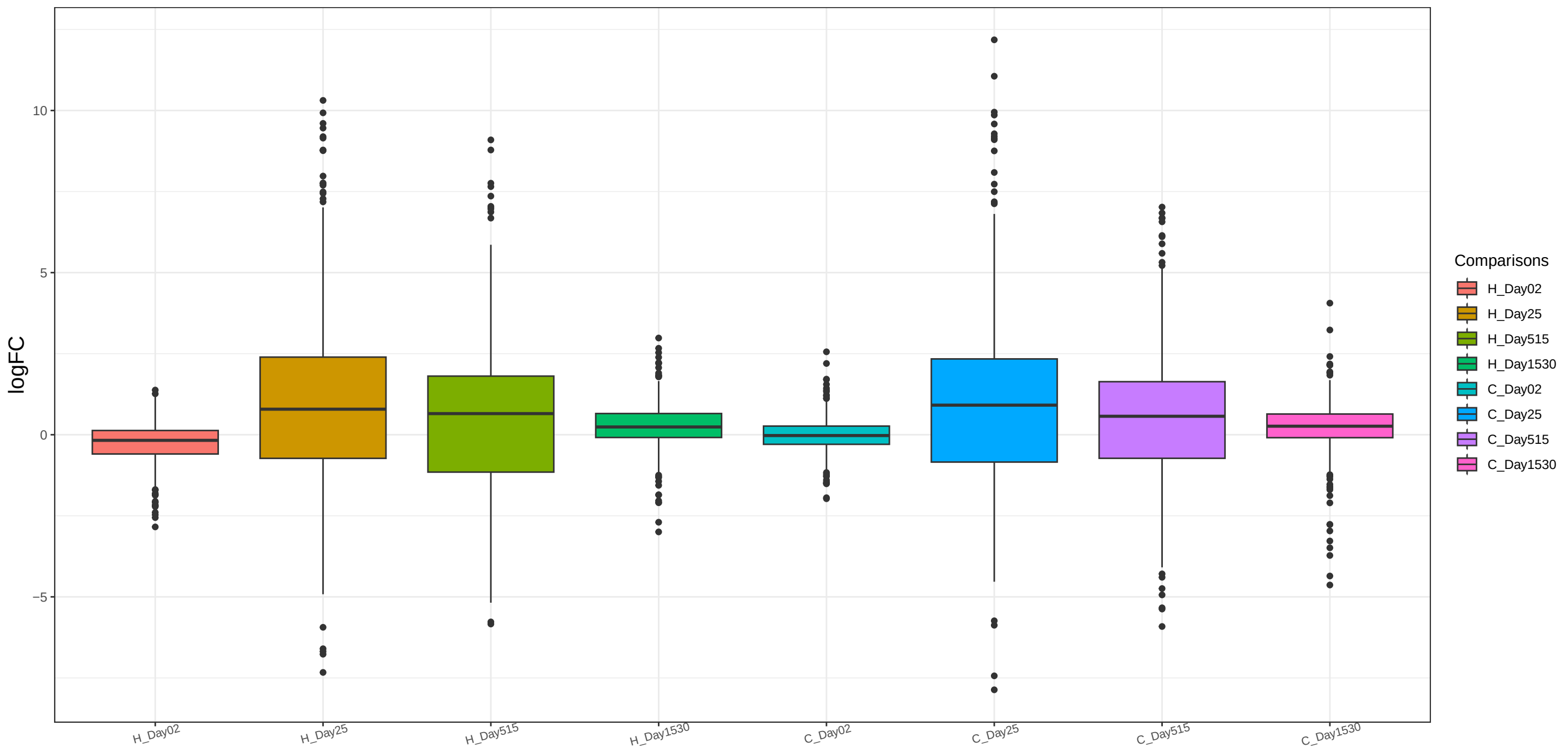
clust4 RNA FC Comparisons Kruskal-Wallis p = 3.89\text{e-}39
