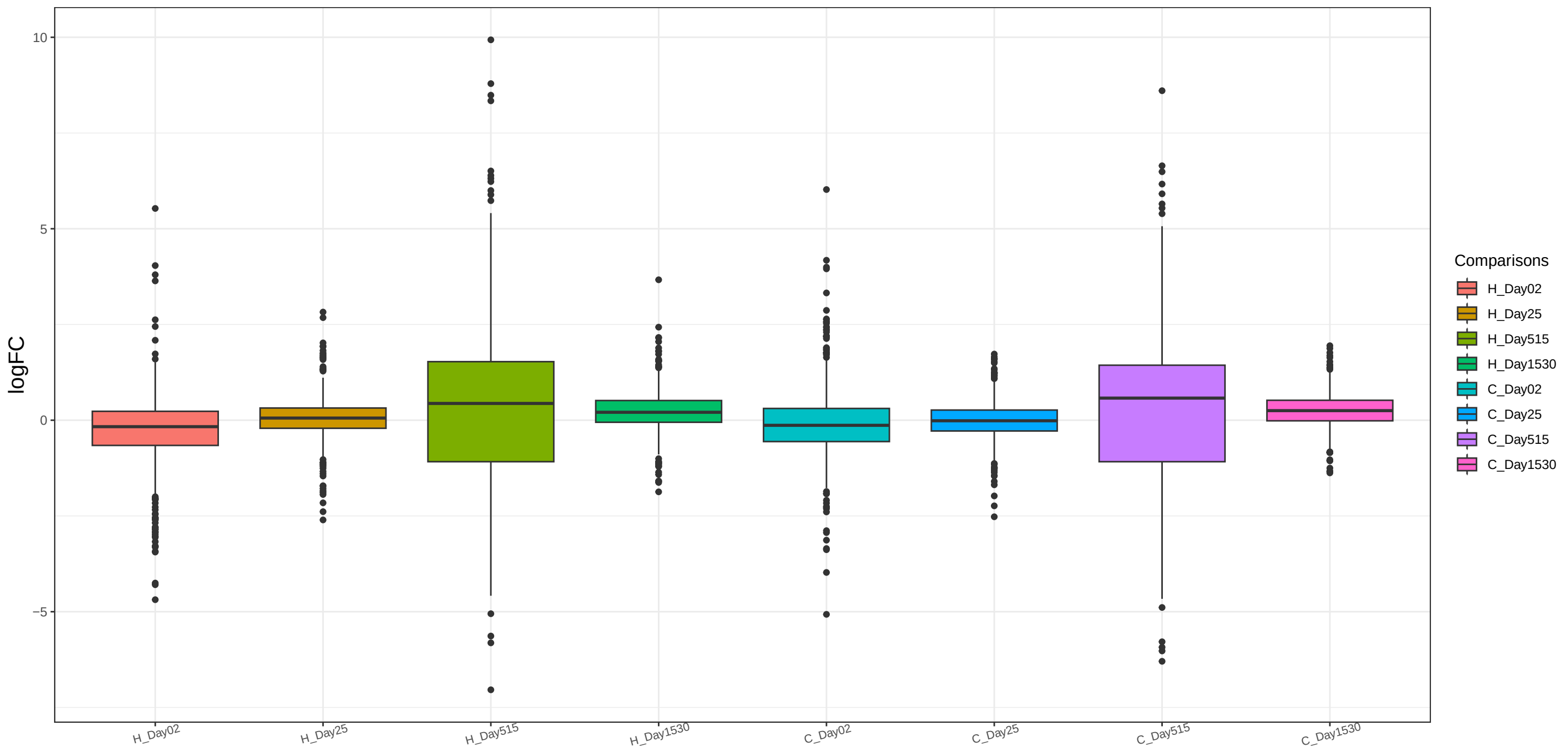
clust5 RNA FC Comparisons Kruskal-Wallis p = 1.47e-48
