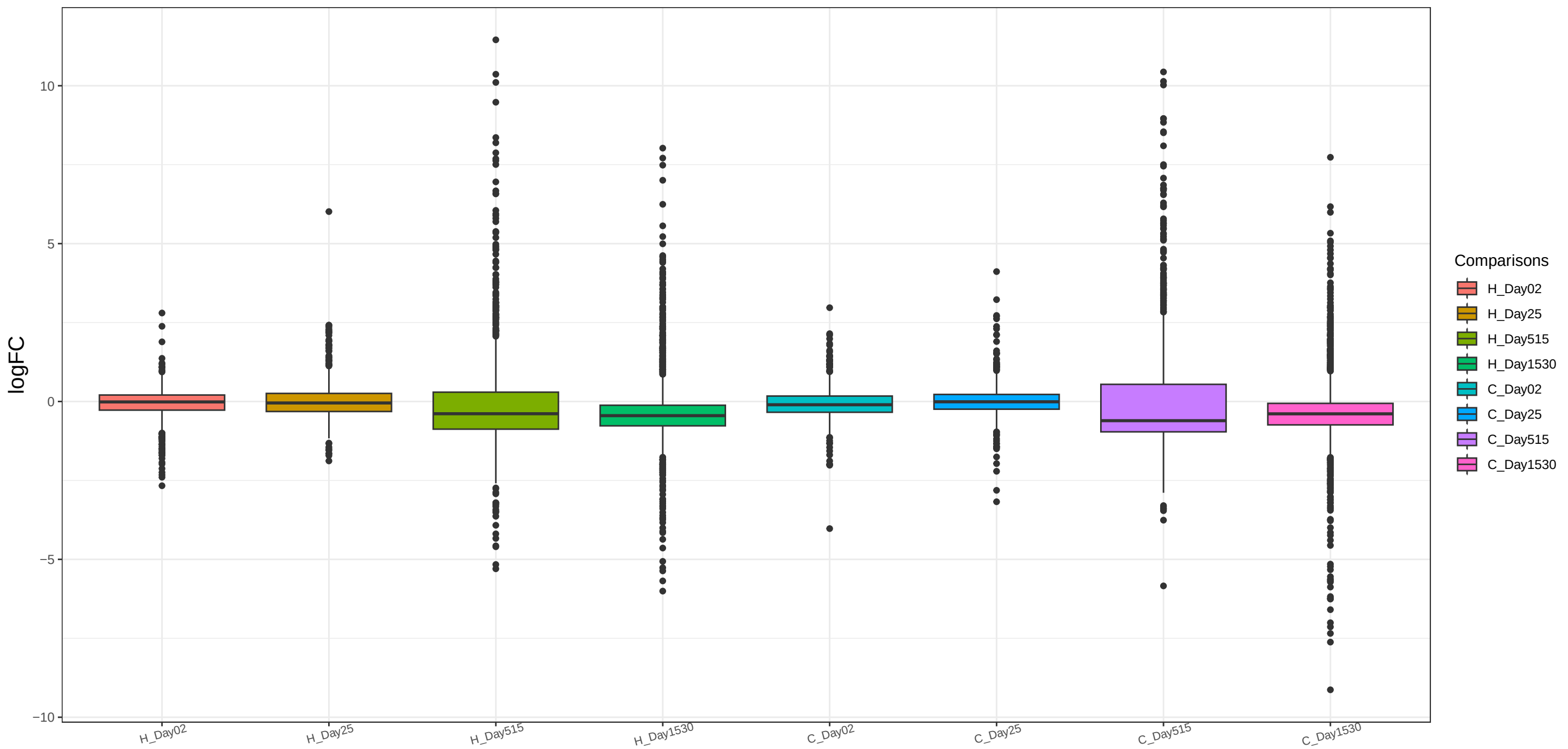
clust7 RNA FC Comparisons Kruskal–Wallis p = 3e-155
