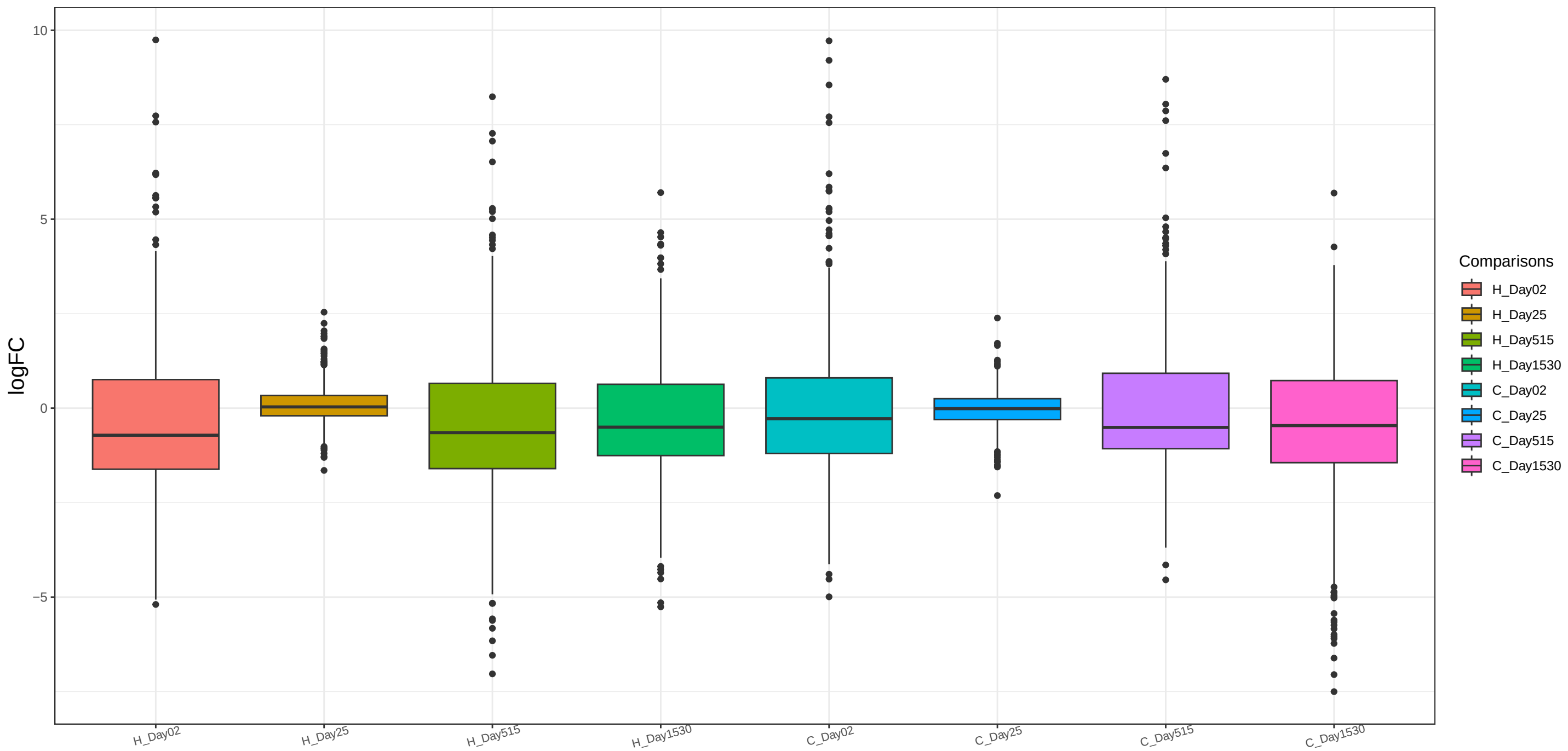
clust8 RNA FC Comparisons Kruskal-Wallis p = 3.04e-29
