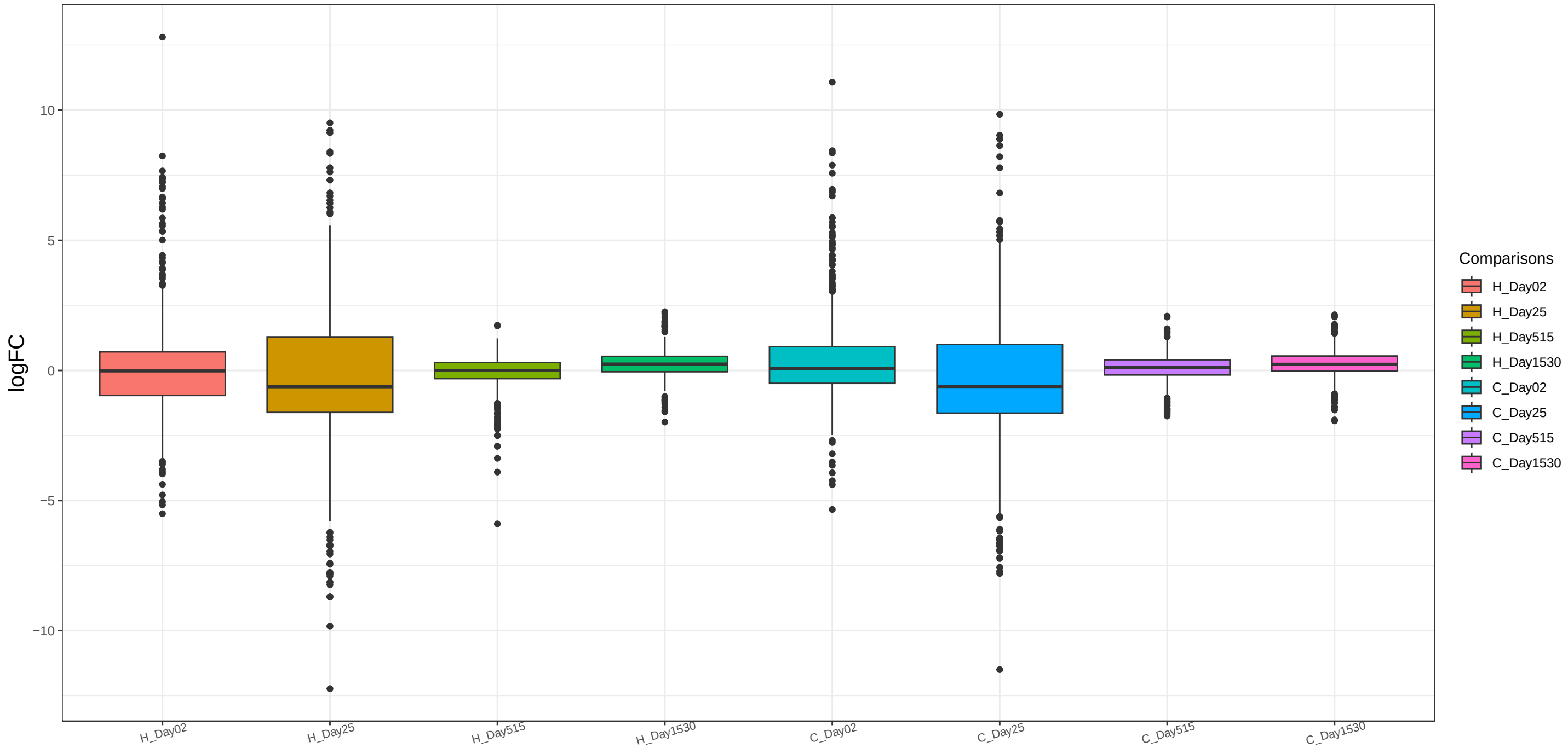
clust9 RNA FC Comparisons Kruskal–Wallis p = 3.14e-37
