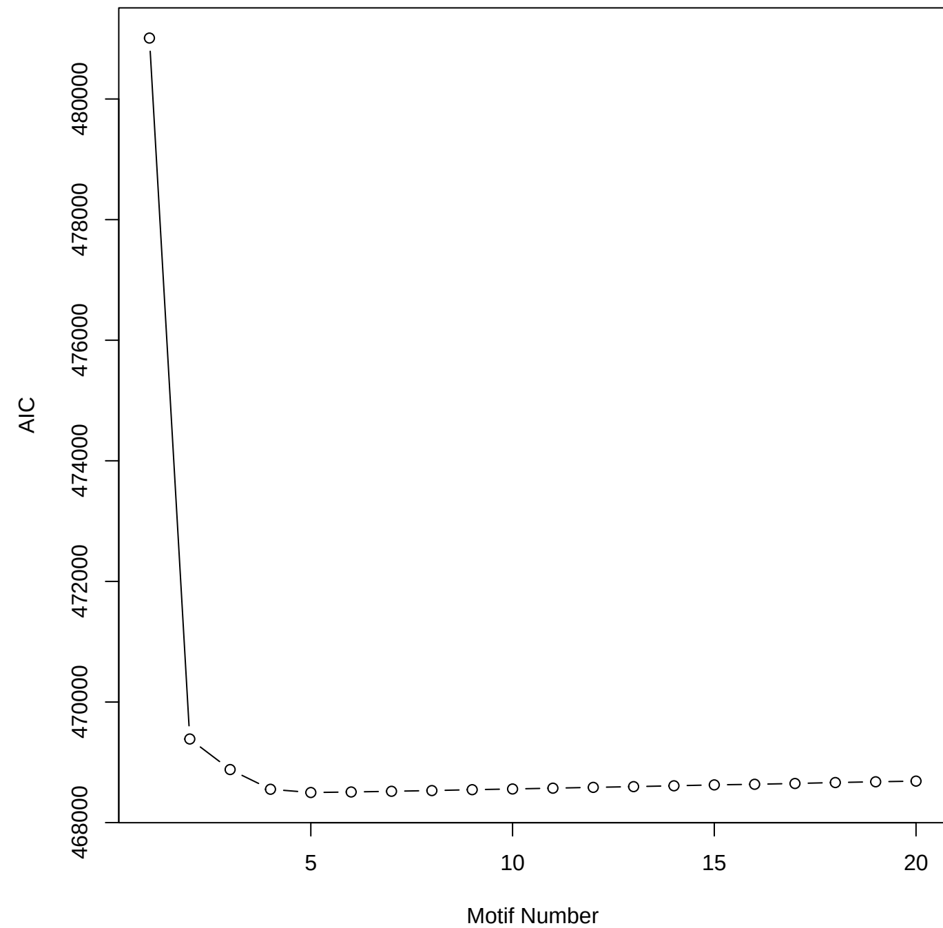
AIC
