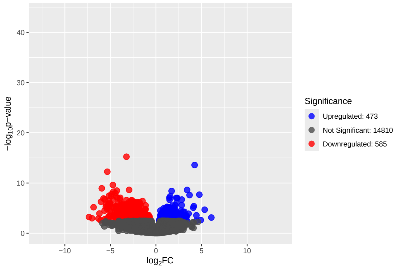
Sig_Sp_inter_Traj515
