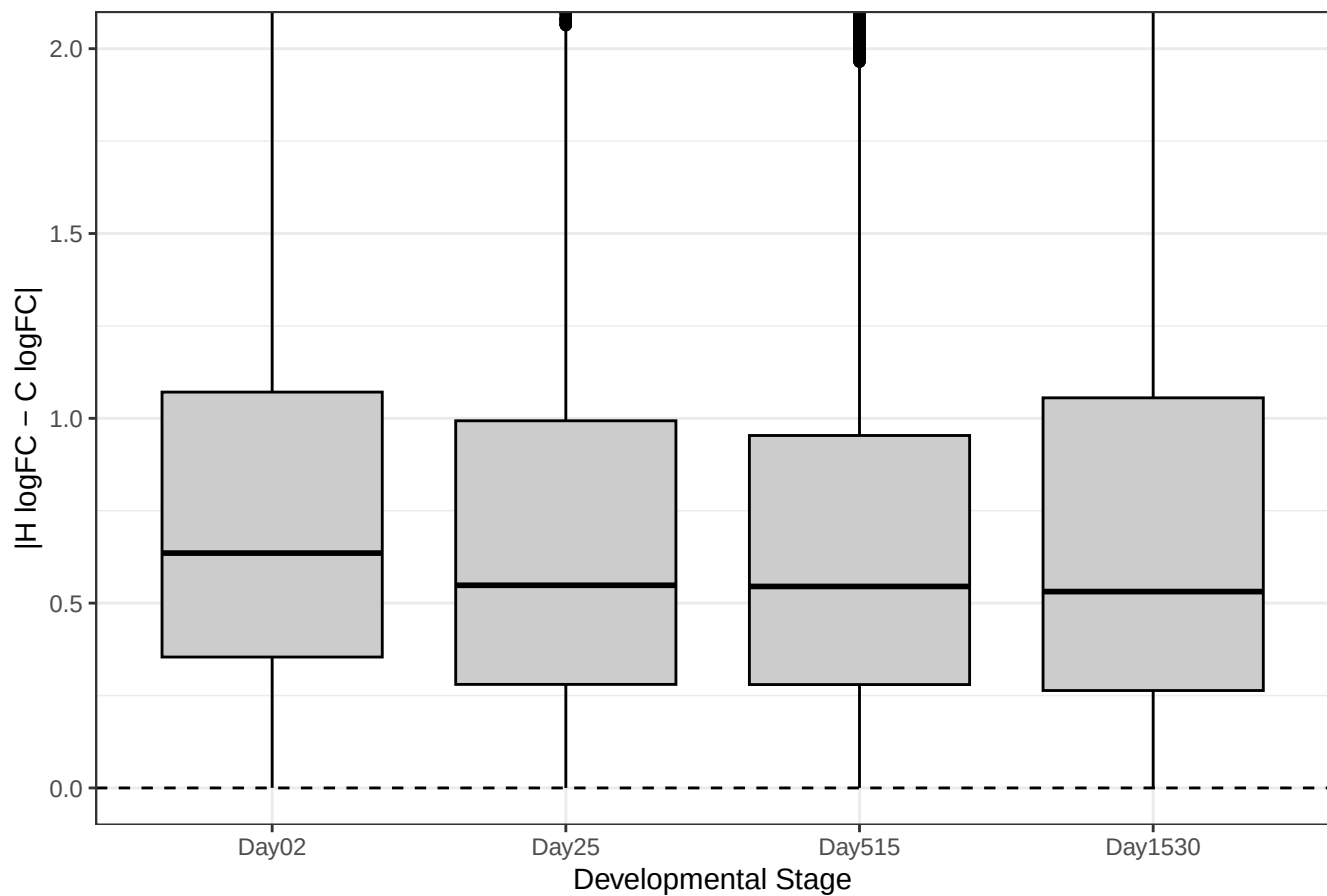
Species divergence across all Trajectory DEGs
