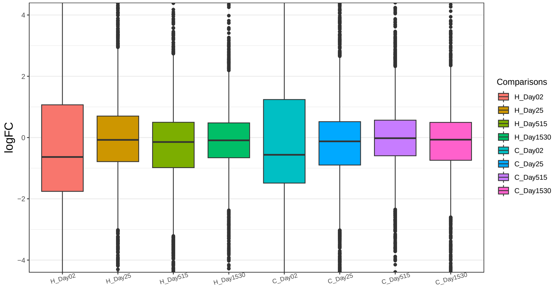
Traj02_genes Trajectory DEG FC Comparisons Kruskal-Wallis p = 1.15e-13
