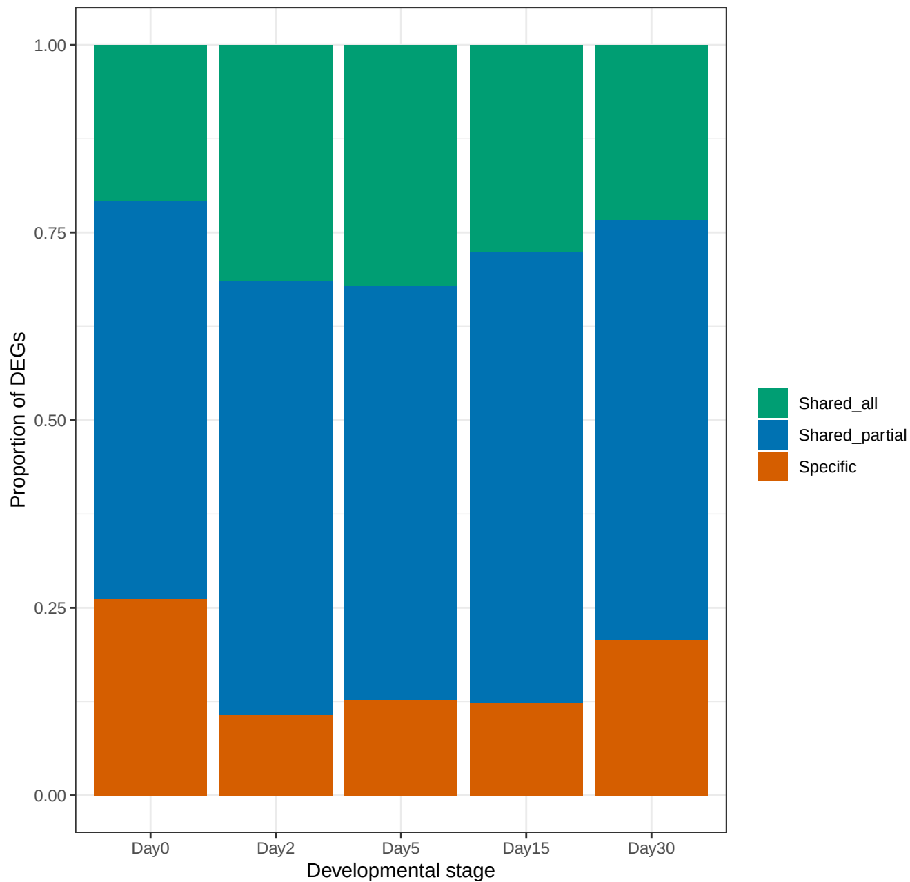
Fate of HVC DEGs across development (normalized)
