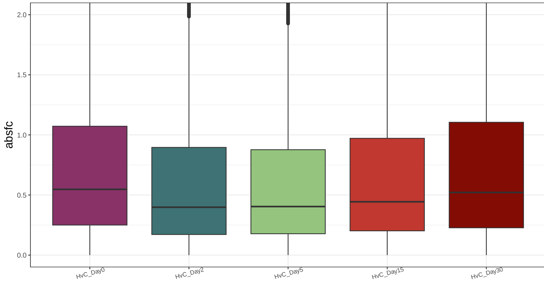
All_Expressed Species DEG absfc Comparisons Kruskal-Wallis p = 1.67\text{e-}55
