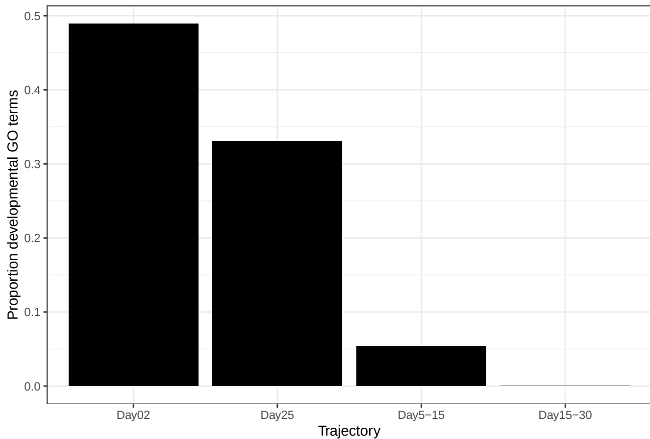
GO enrichment of DEGs (All)
