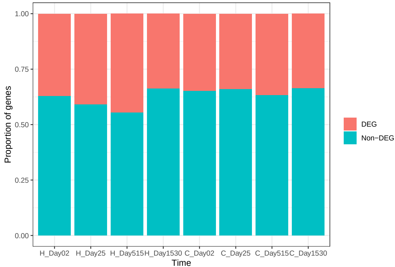
DEG vs NonDEG composition
