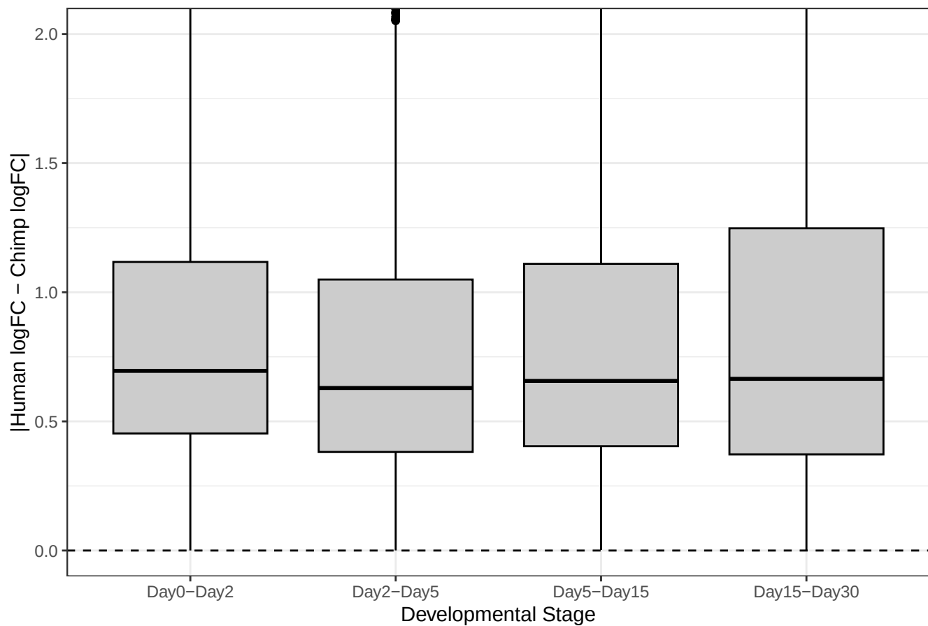
Species divergence in species-specific DEGs
