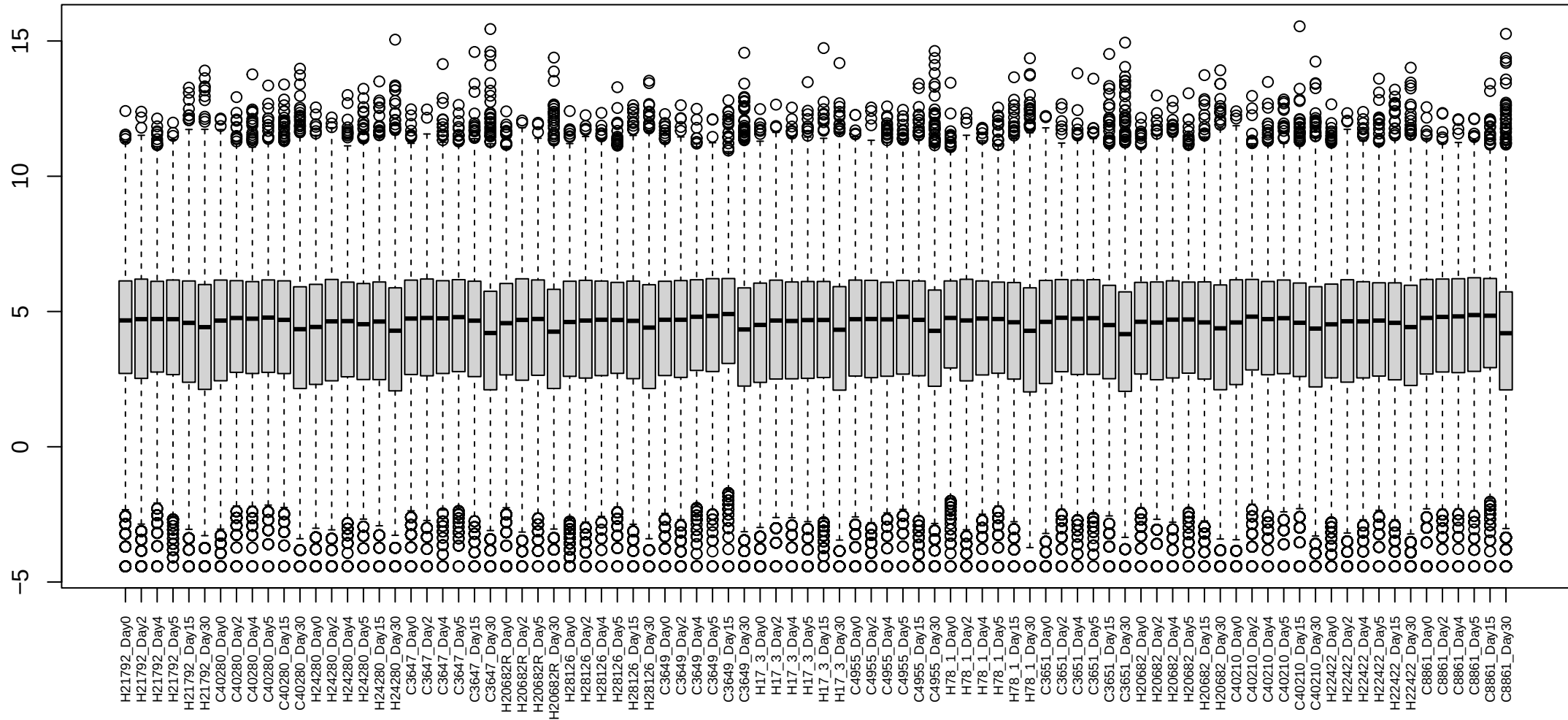
Boxplots of log cpm per sample (RowMeans>0)
