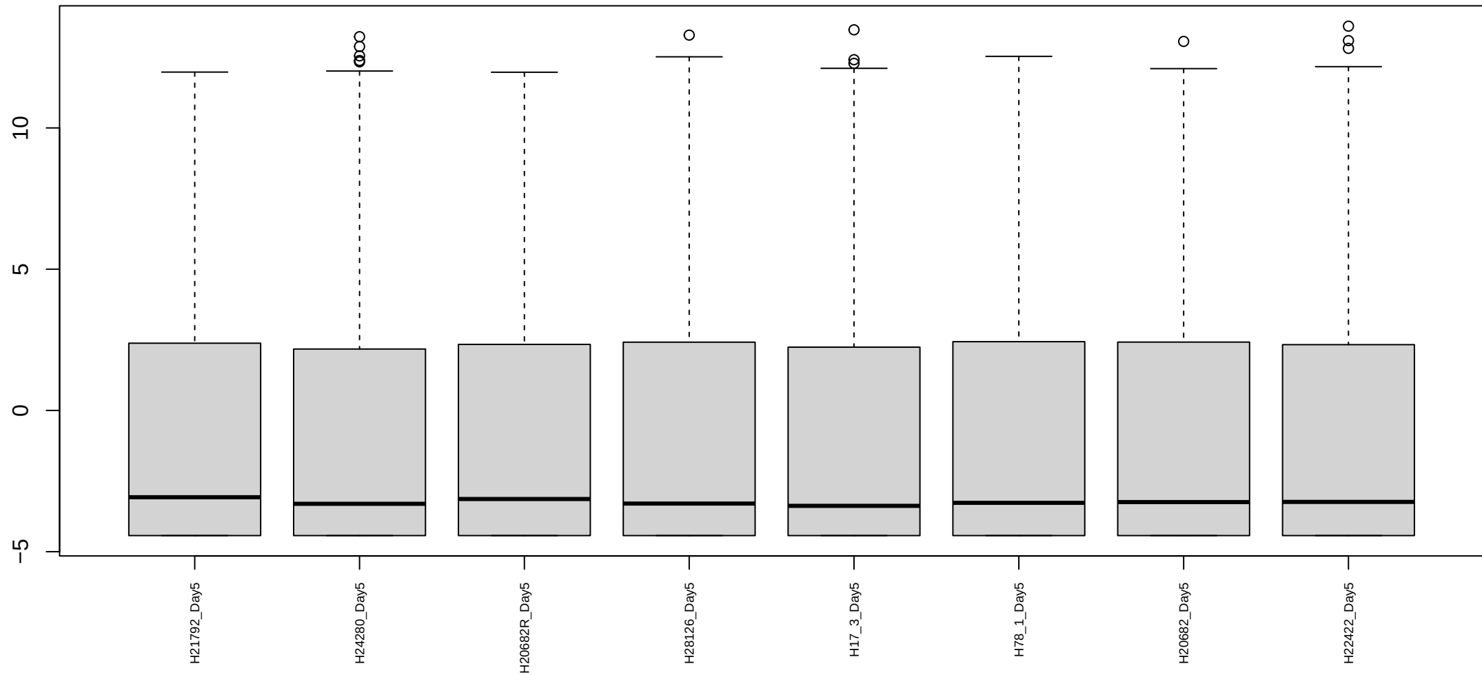
Boxplots of log cpm per sample Human Day 5 (unfiltered)
