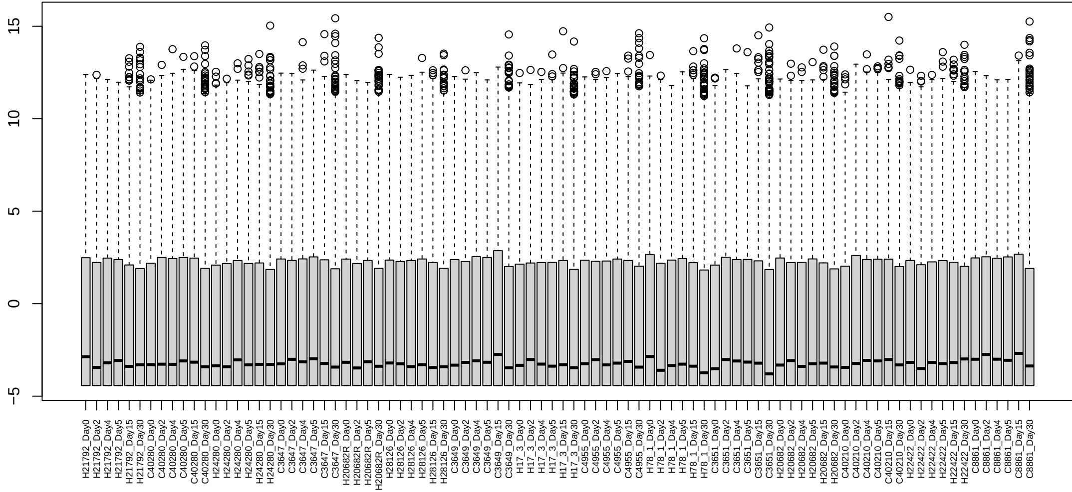
Boxplots of log cpm per sample (unfiltered)
