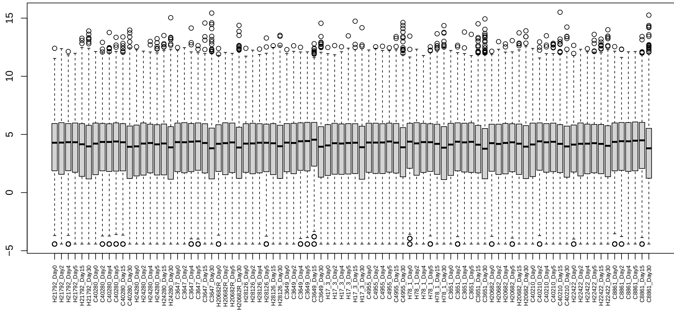
Boxplots of log cpm per sample with lcpm >1 in 4/7 species-timepoints
