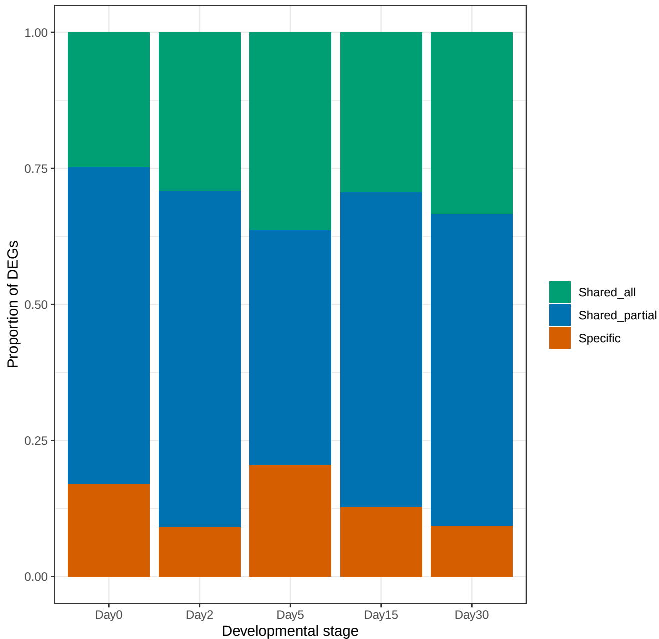
Fate of HvC KZFP DEGs across development (normalized)
