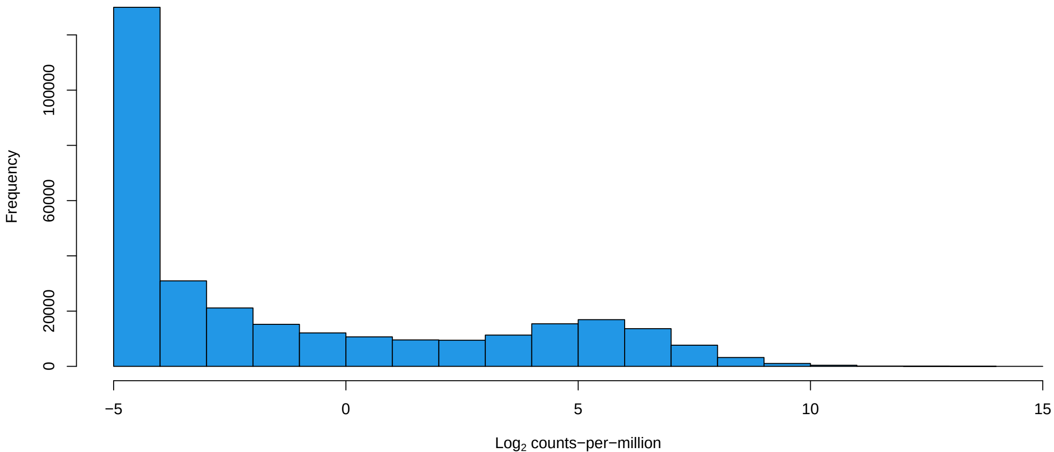
Histogram of all counts – Human Day 15 (unfiltered)
