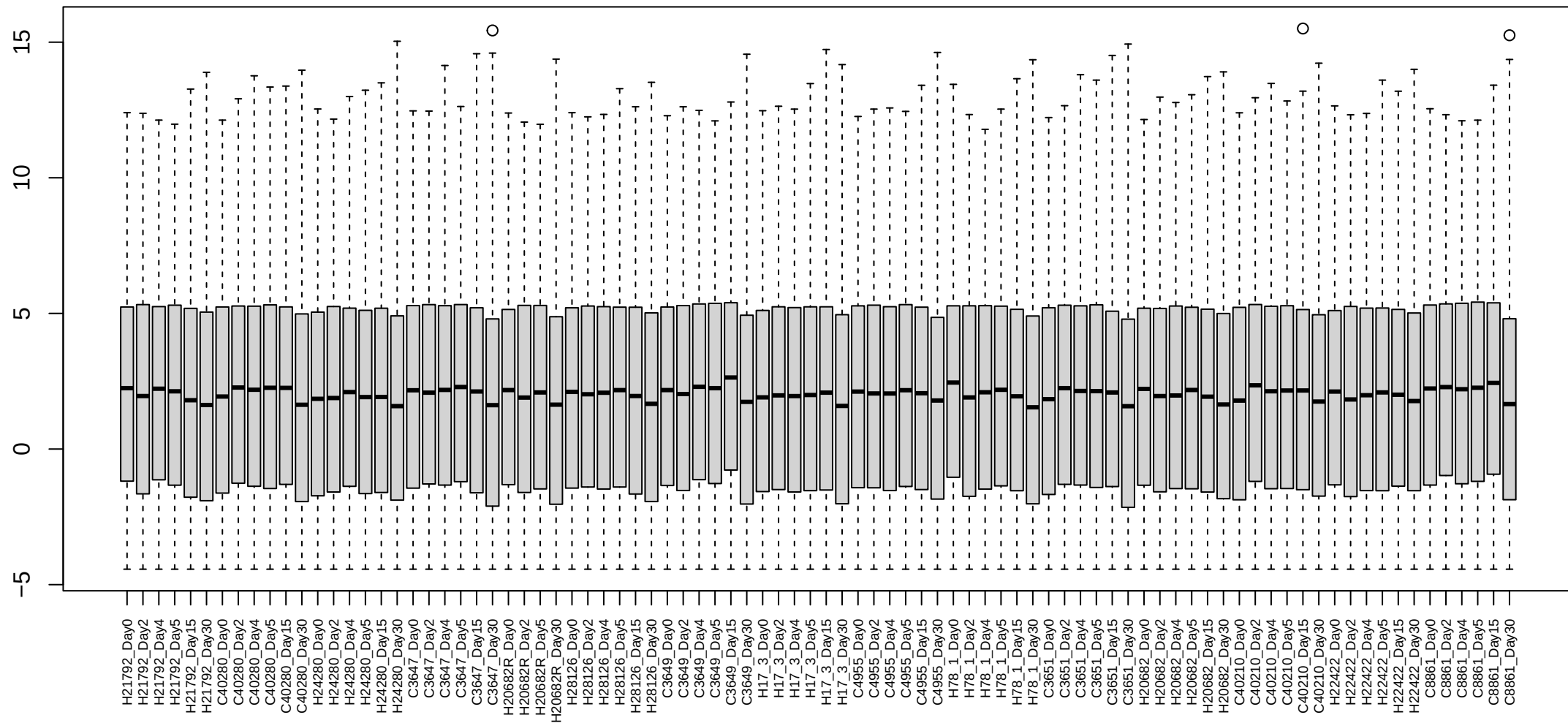
Boxplots of log cpm EdgeR FilterByExpression
