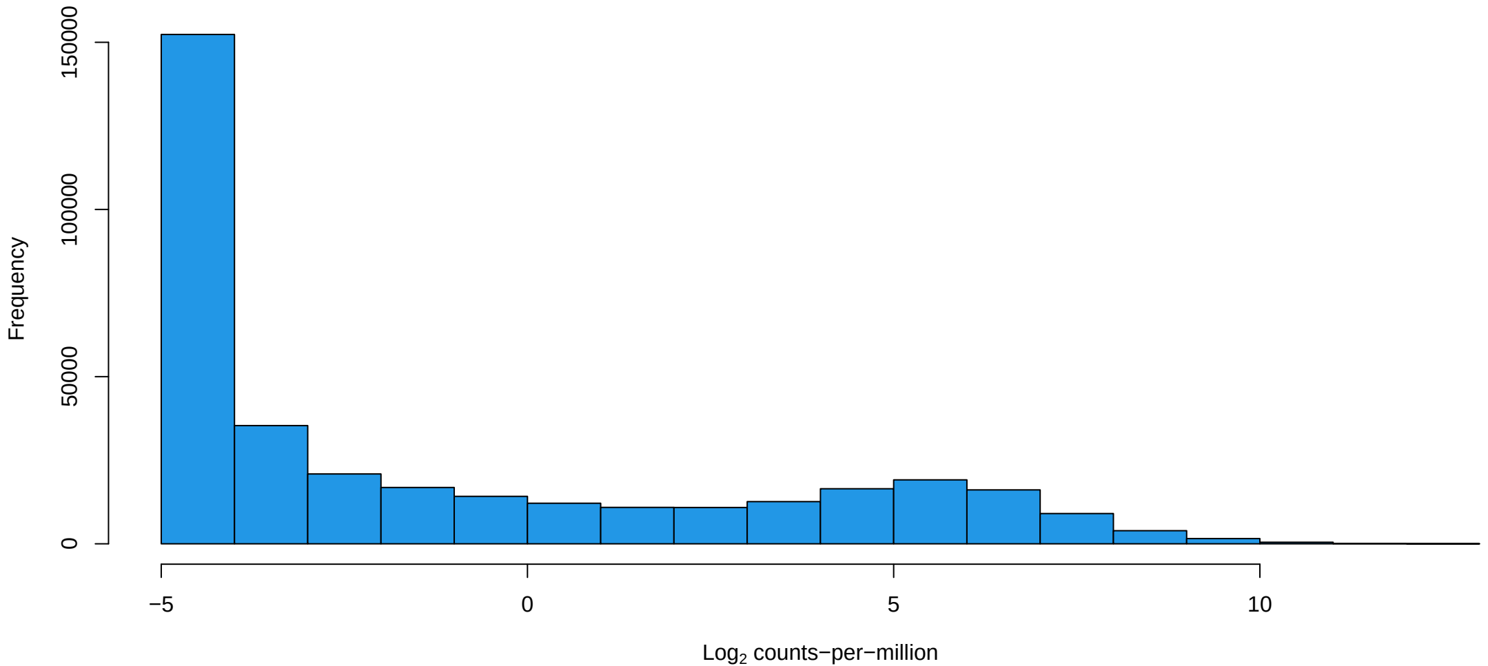
Histogram of all counts – Human Day 2 (unfiltered)
