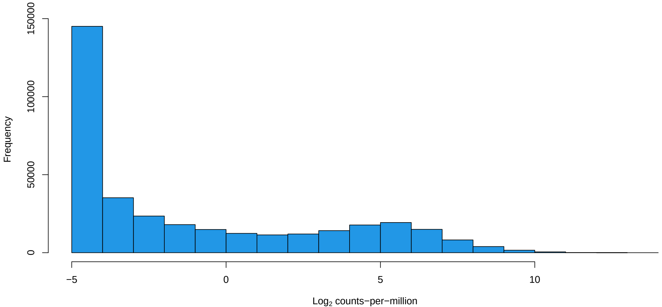
Histogram of all counts – Human Day 0 (unfiltered)
