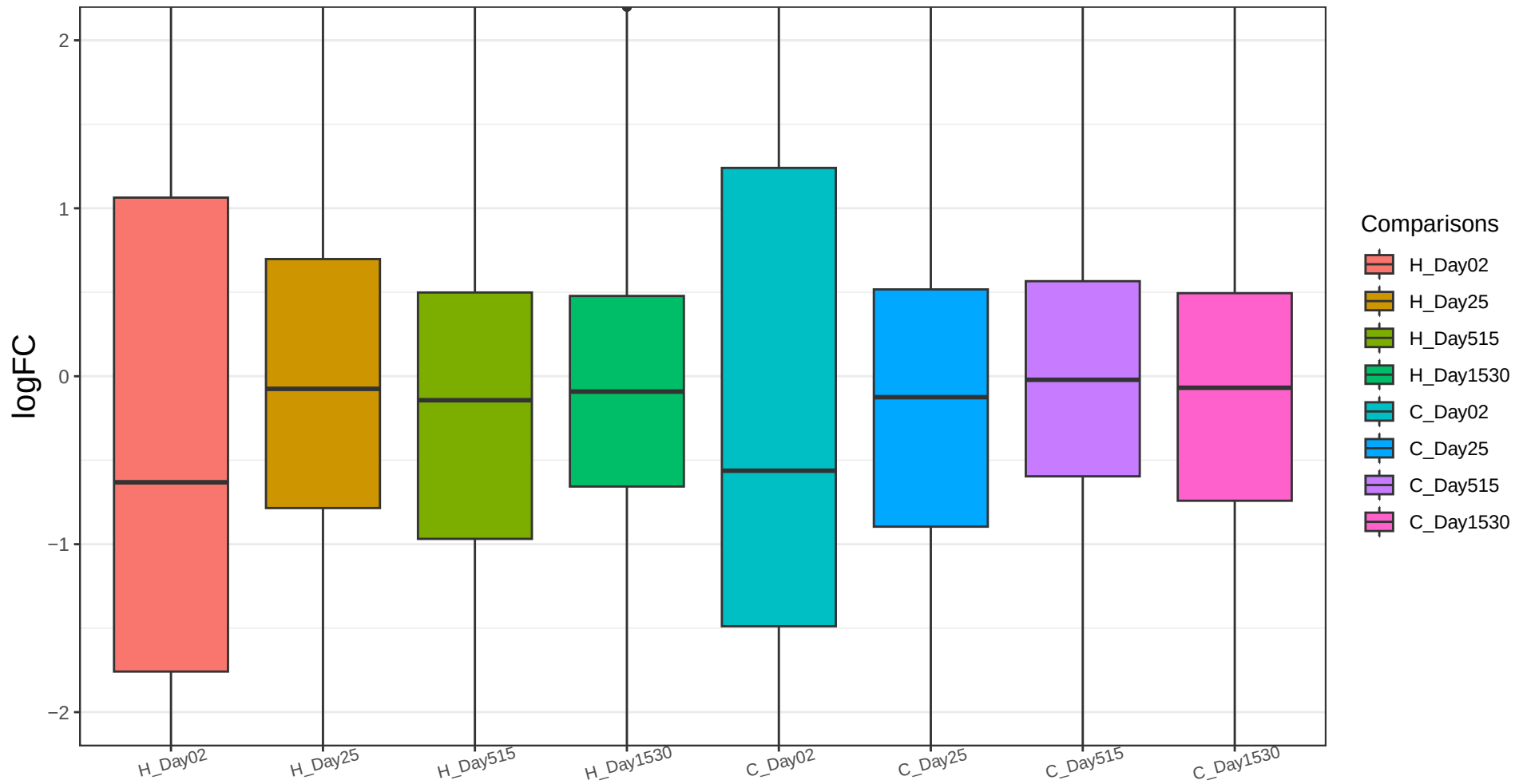
Traj02_genes Trajectory DEG FC Comparisons Kruskal-Wallis p = 1.75e-13
