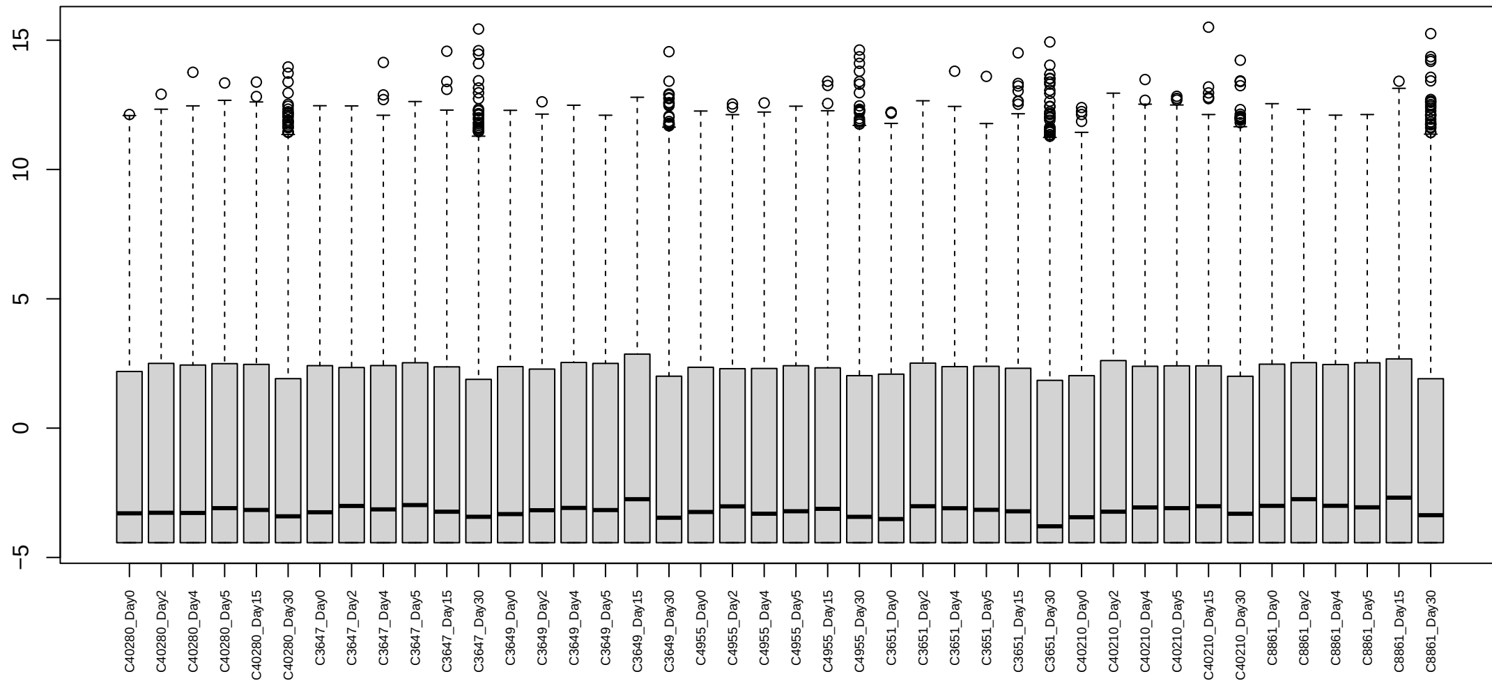
Boxplots of log cpm per sample – Chimp (unfiltered)
