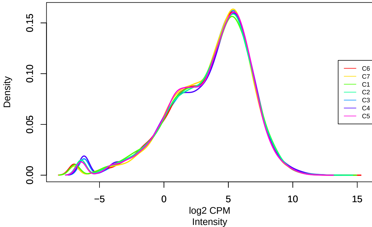
C Day4
