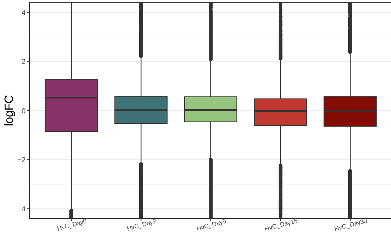
HvC_Day0_all Species DEG FC Comparisons Kruskal-Wallis p = 1.69\text{e-}34
