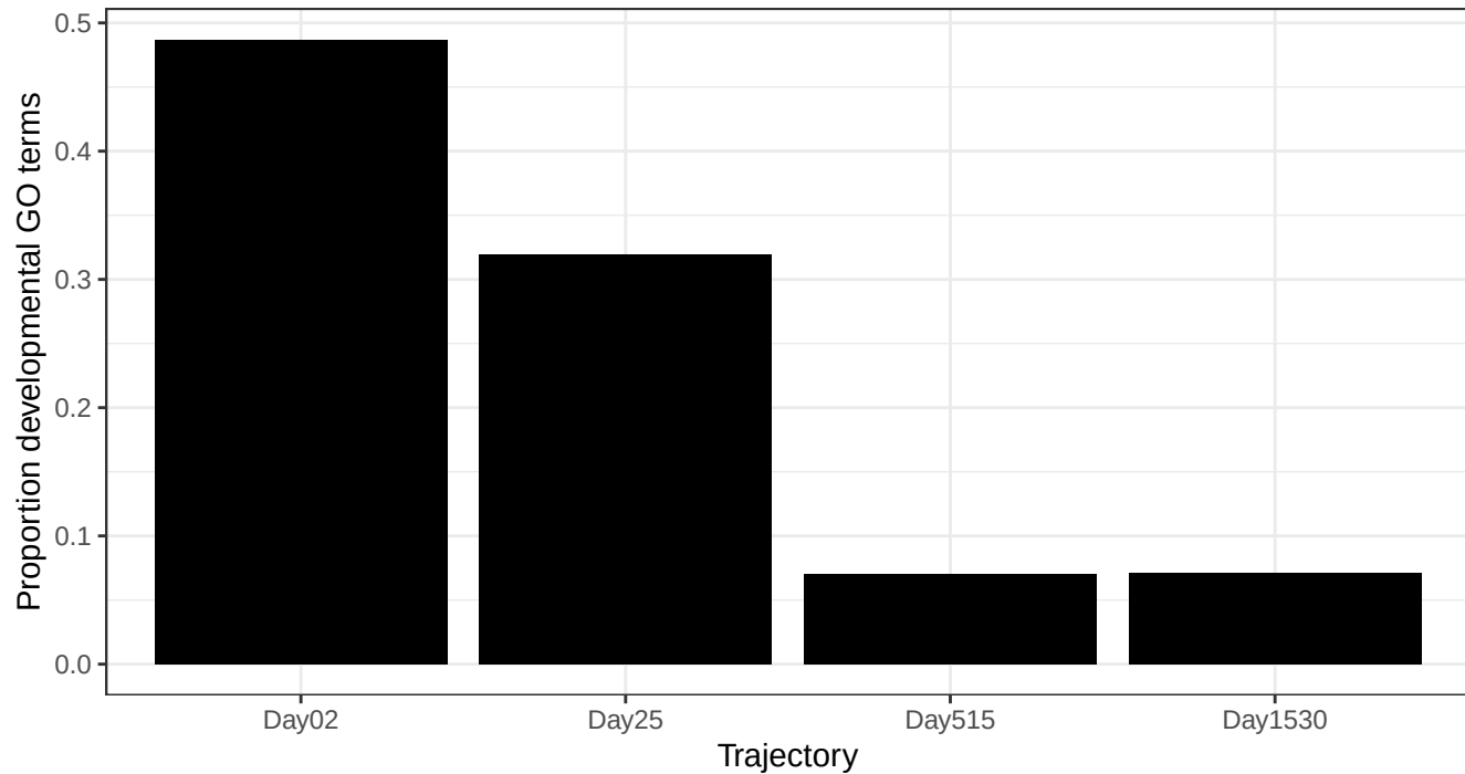
GO enrichment of DEGs (All DEGs at a transition)
