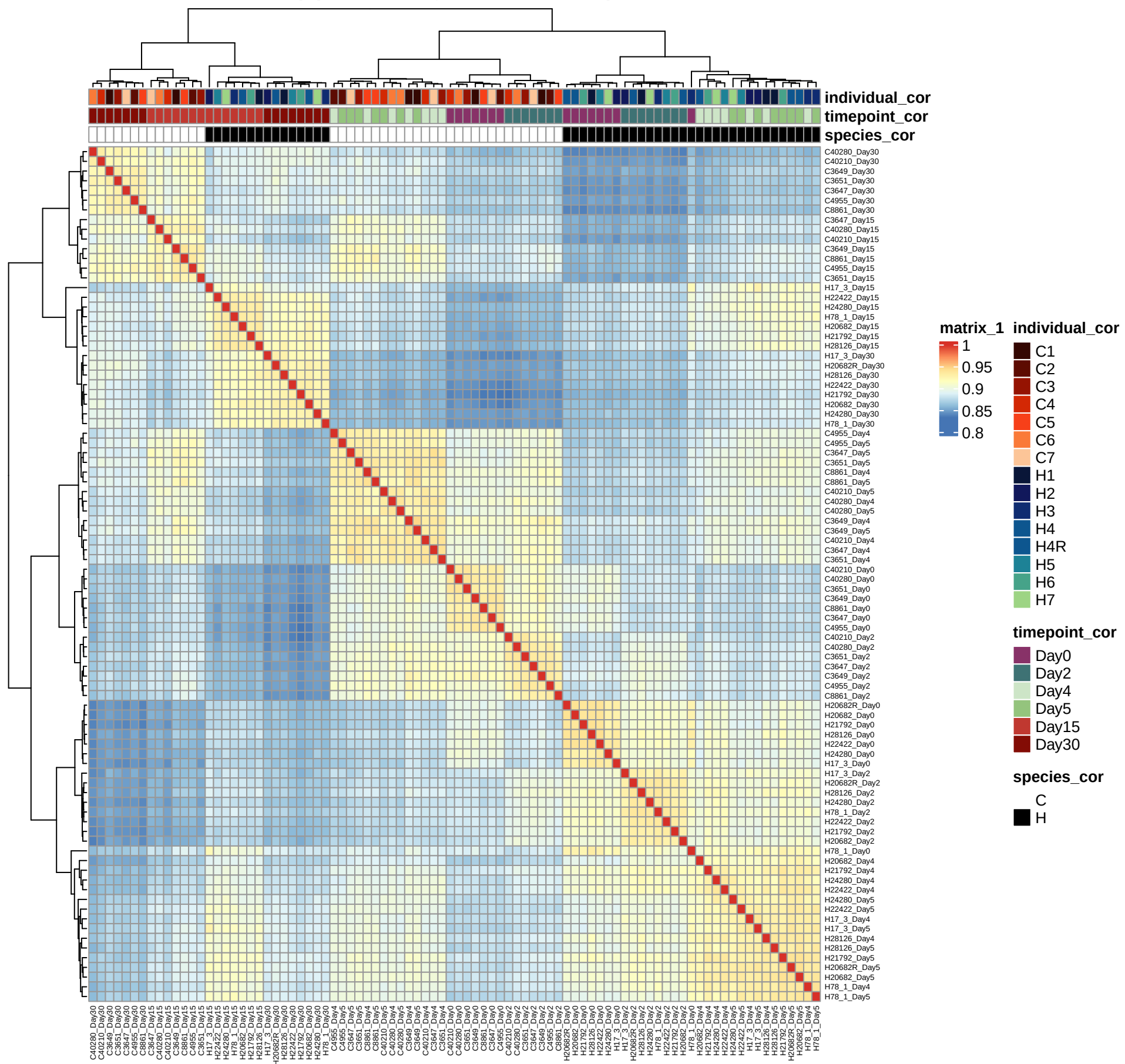
Sample-Sample Correlation (Spearman-log2CPM-Unfiltered)
