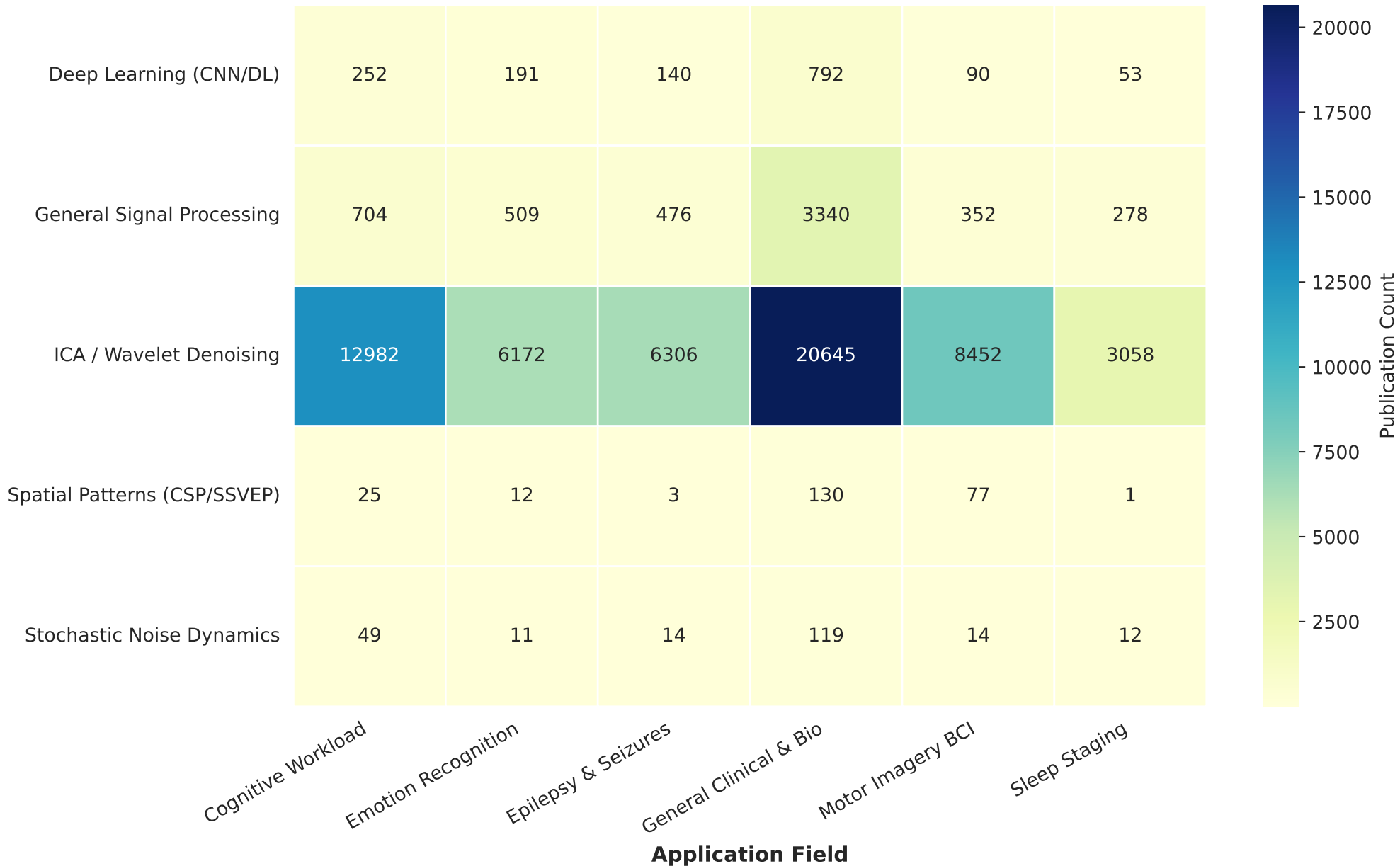
Methodology vs Application Field Cross-Tabulation Matrix
